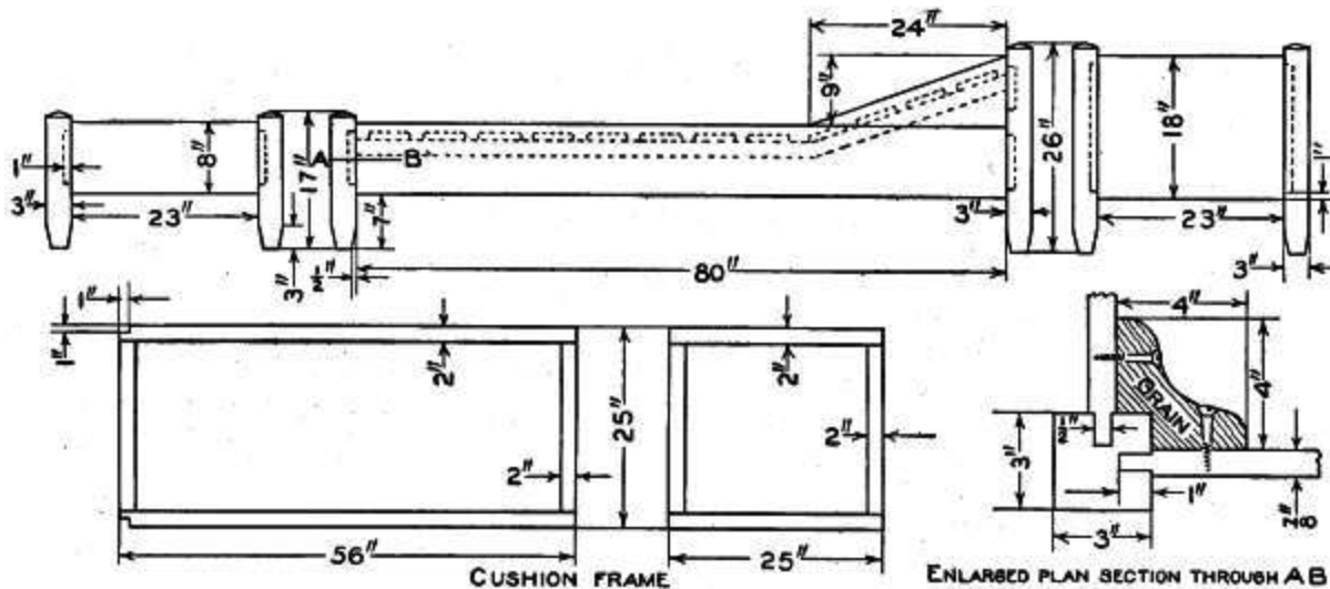
Details of Mission Couch
