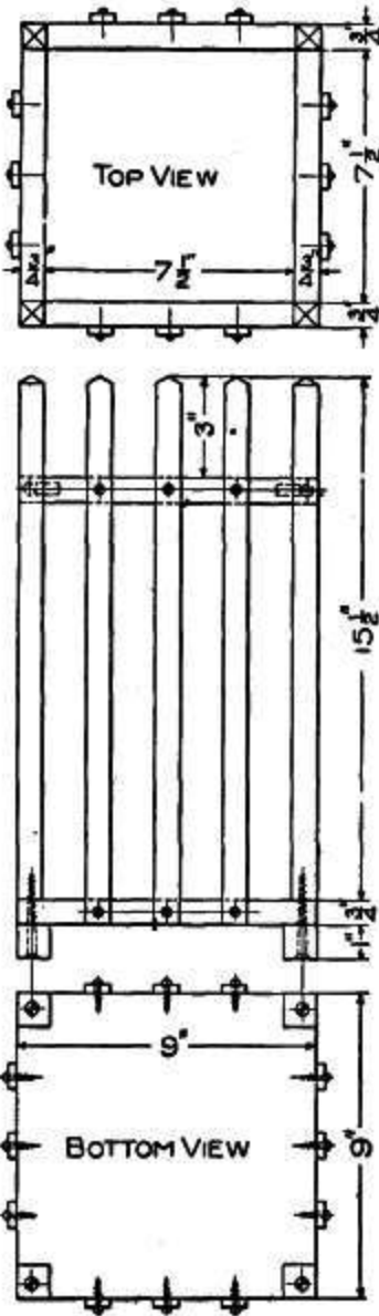
DETAILS OF WASTE PAPER BASKET
