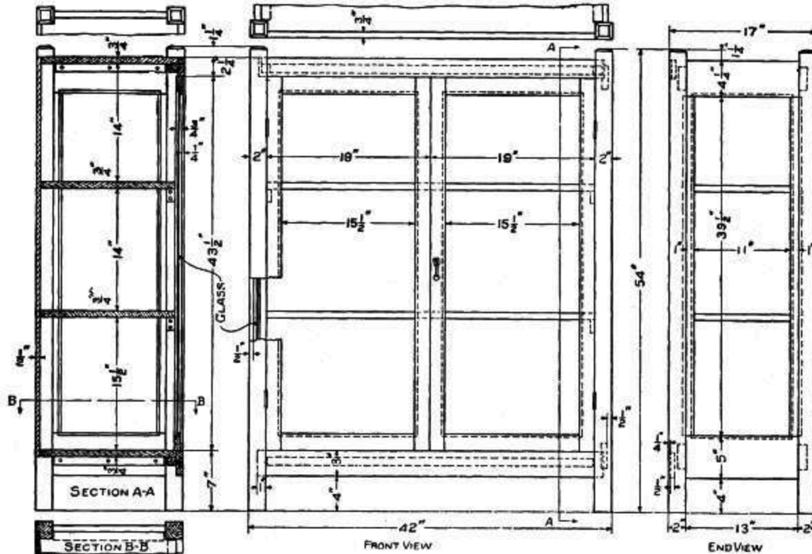
Details of China Closet
