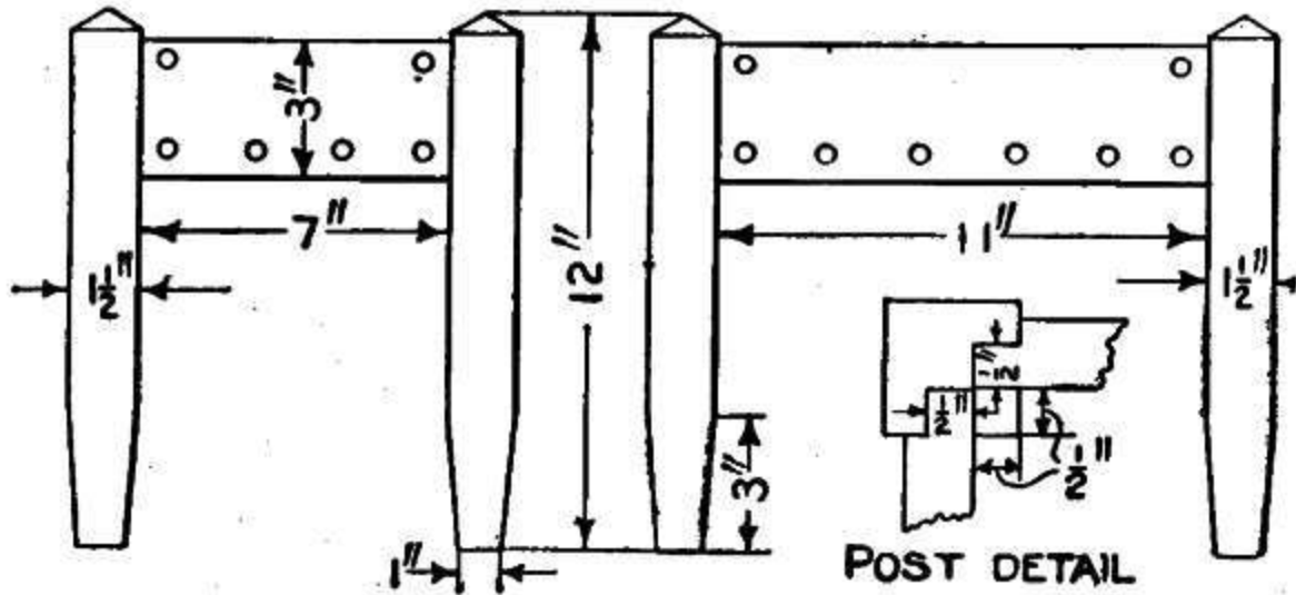
Details of Footstool
