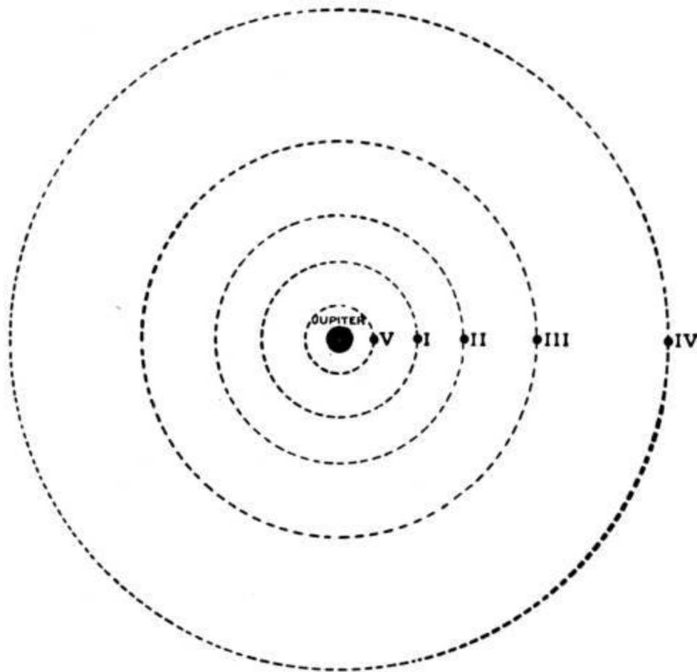
FIG. 93.—Jupiter and its satellites.
