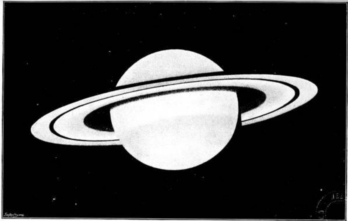
FIG. 95.—Saturn and its rings. From a drawing by Professor Barnard.
