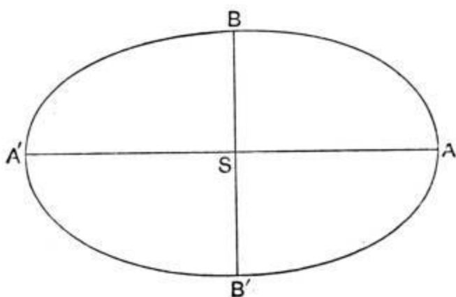
FIG. 76.—The aberrational ellipse.
