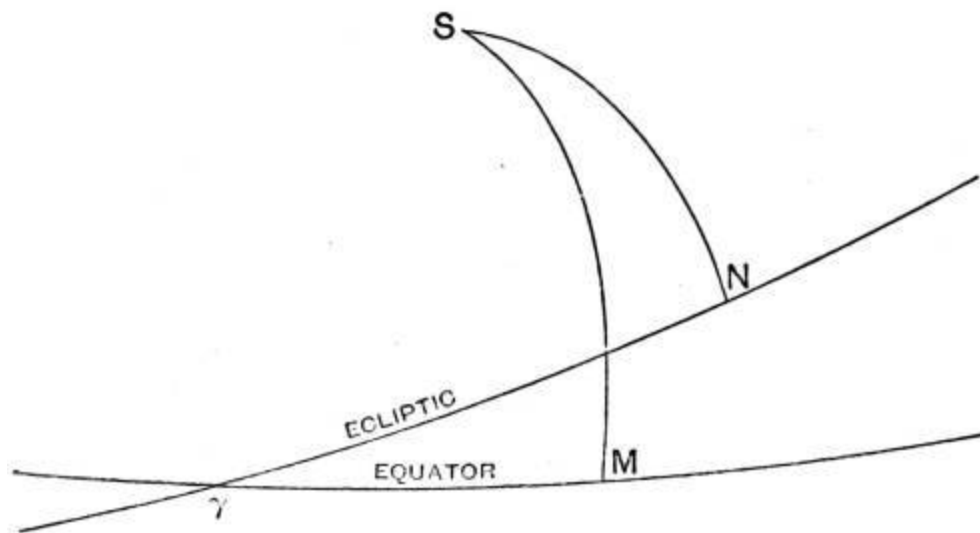
FIG. 14.—The equator and the ecliptic.
