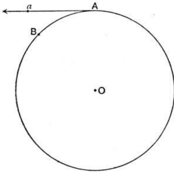
FIG. 70.—Motion in a circle.
