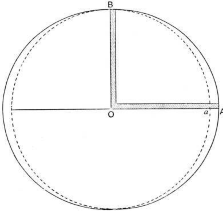
FIG. 72.—The spheroidal form of the earth.
