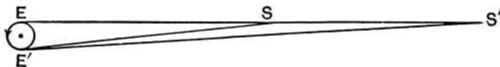
FIG. 50.—Stellar parallax.
