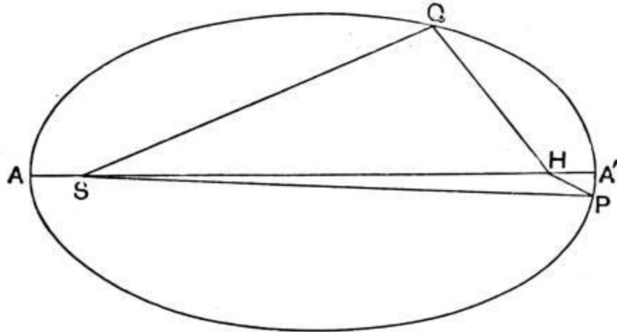
FIG. 59.—An ellipse.
