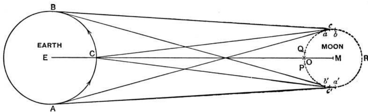
FIG. 58.—The daily libration of the moon.
