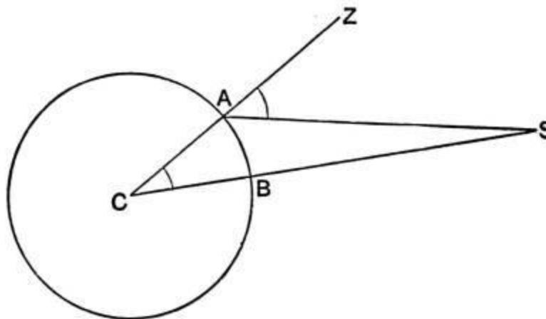
FIG. 16.—The measurement of the earth.
