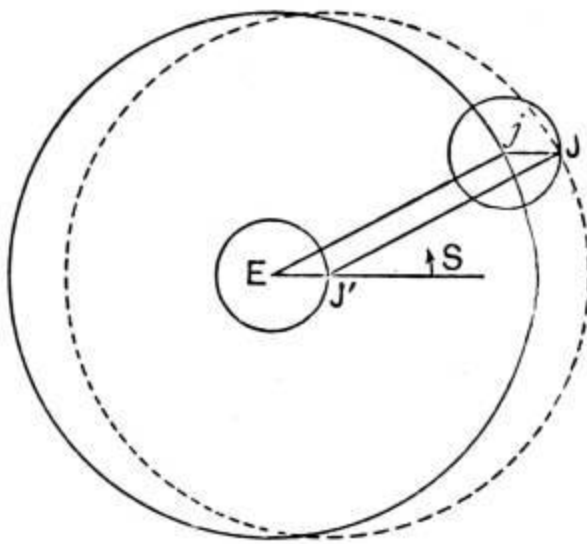
FIG. 45.—The epicycle of Jupiter.
