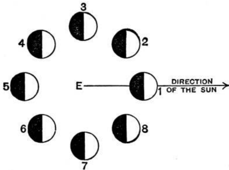
FIG. 10.—The phases of the moon.
