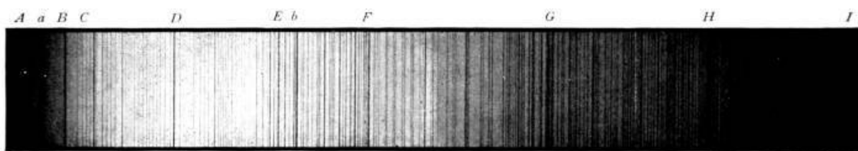
FIG. 97.—Fraunhofer's map of the solar spectrum. (The red end of the spectrum is on the left, the violet on the right.)
