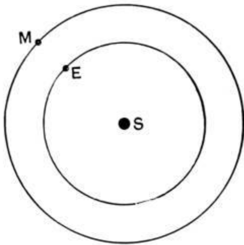
FIG. 68.—Mars in opposition.
