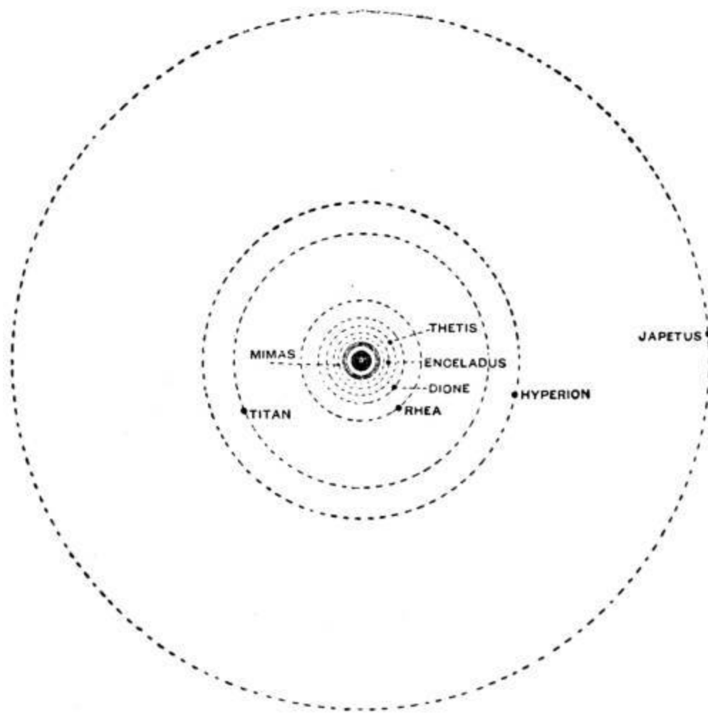
FIG. 91.—Saturn and its system.
