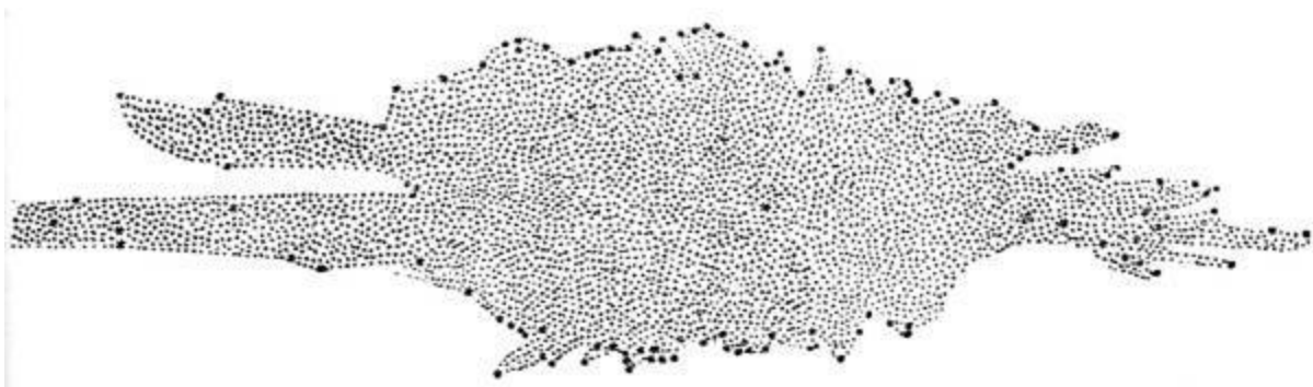
FIG. 83.—Section of the sidereal system. From Herschel's paper in the Philosophical Transactions .
