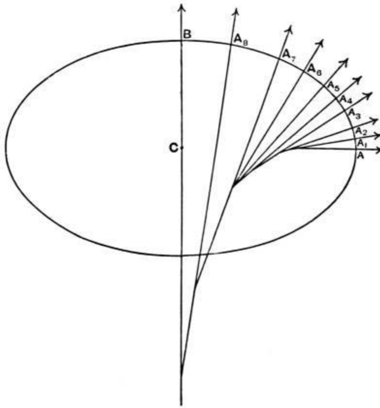
FIG. 78.—The varying curvature of the earth.
