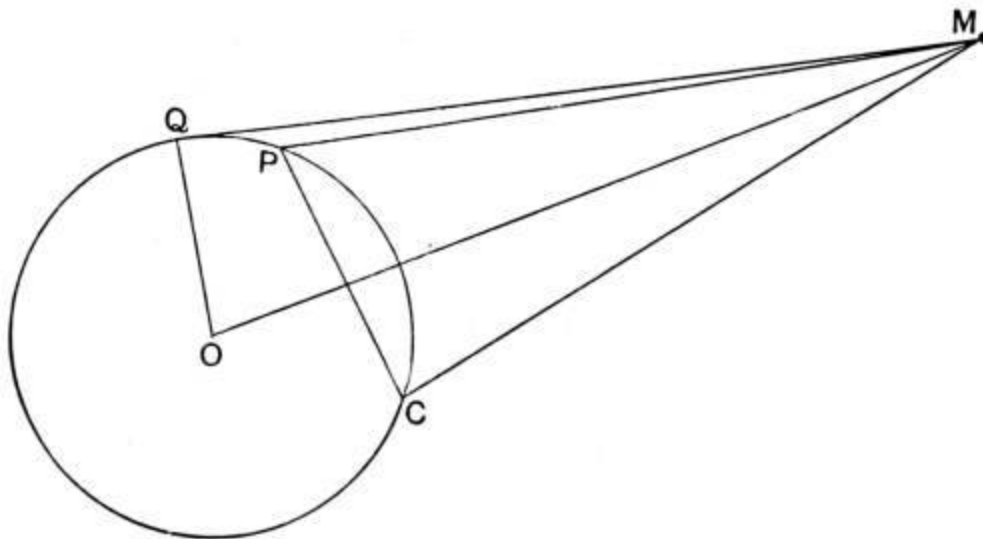
FIG. 69.—The parallax of a planet.
