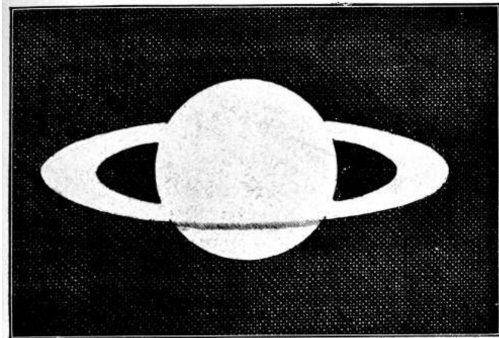
FIG. 64.—Saturn's ring, as drawn by Huygens. From the Systema Saturnium . [To face p. 200.]
