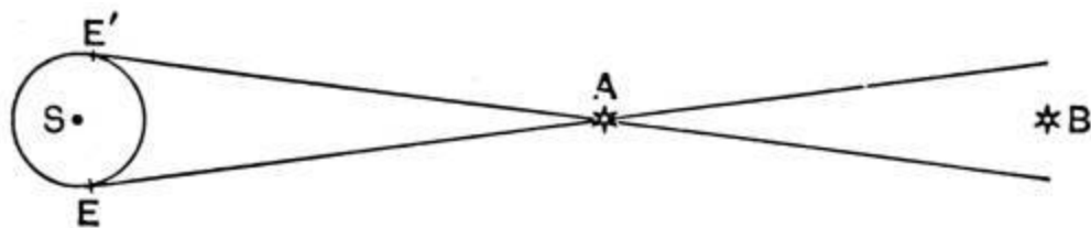
FIG. 57.—The differential method of parallax.
