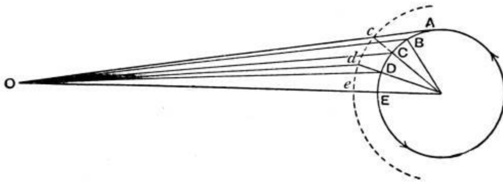
FIG. 56.—Galilei's proof that sun-spots are not planets.
