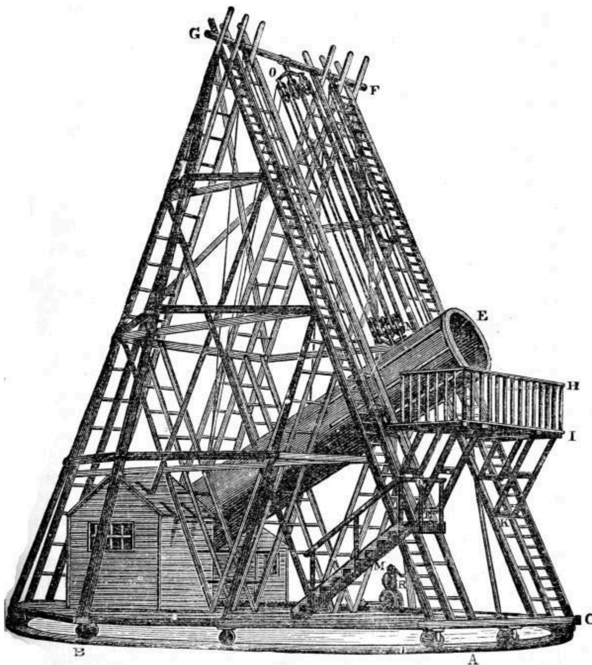
FIG. 82.—Herschel's forty-foot telescope.
