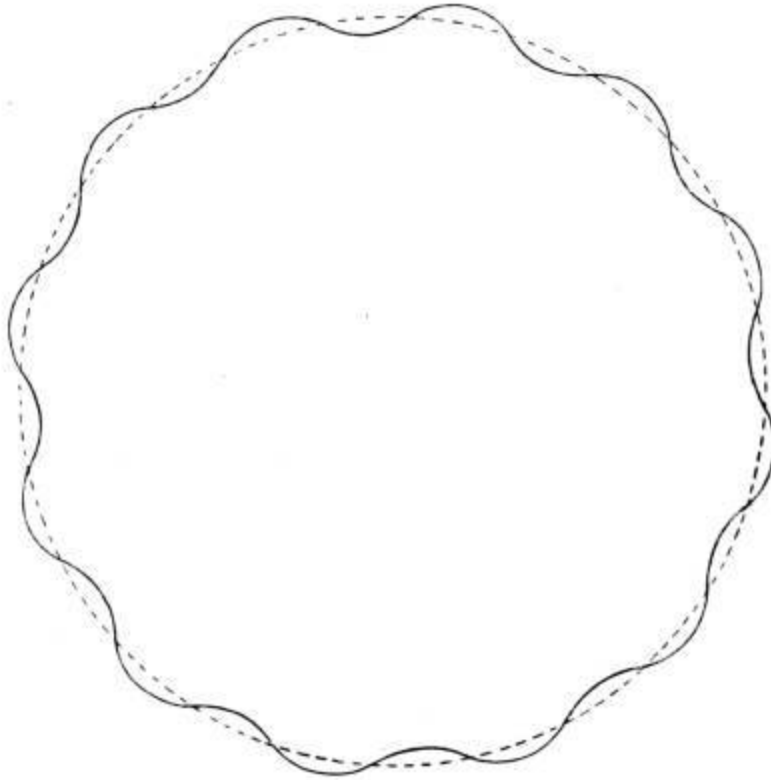
FIG. 77.—Precession and nutation.
