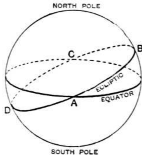
FIG. 4.—The equator and the ecliptic.
