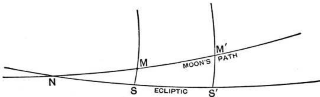
FIG. 26.—The ecliptic and the moon's path.
