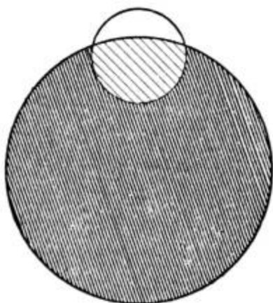
FIG. 28.—Partial eclipse of the moon.
