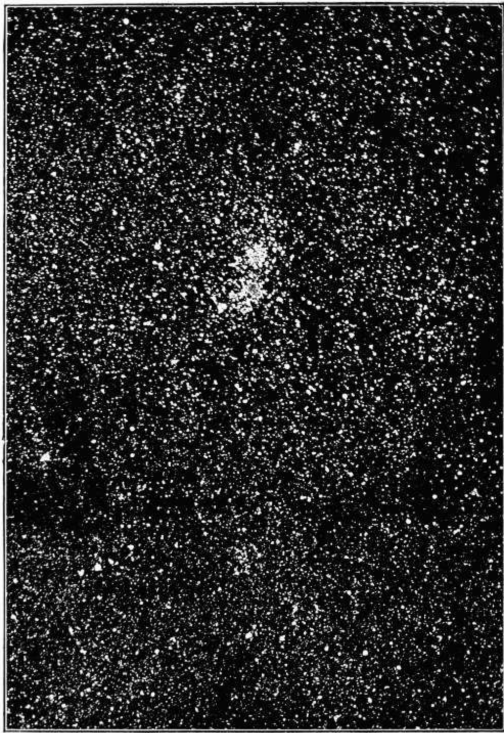
FIG. 104.—The Milky Way near the cluster in Perseus. From a photograph by Professor Barnard.
