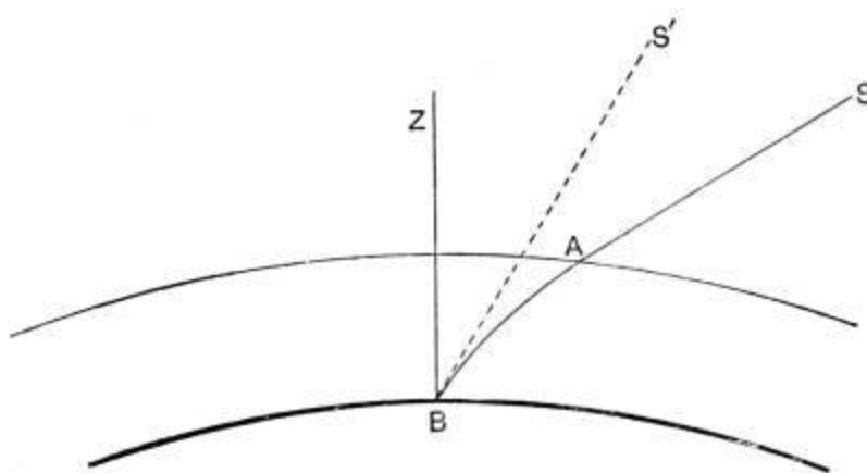
FIG. 32.—Refraction by the atmosphere.
