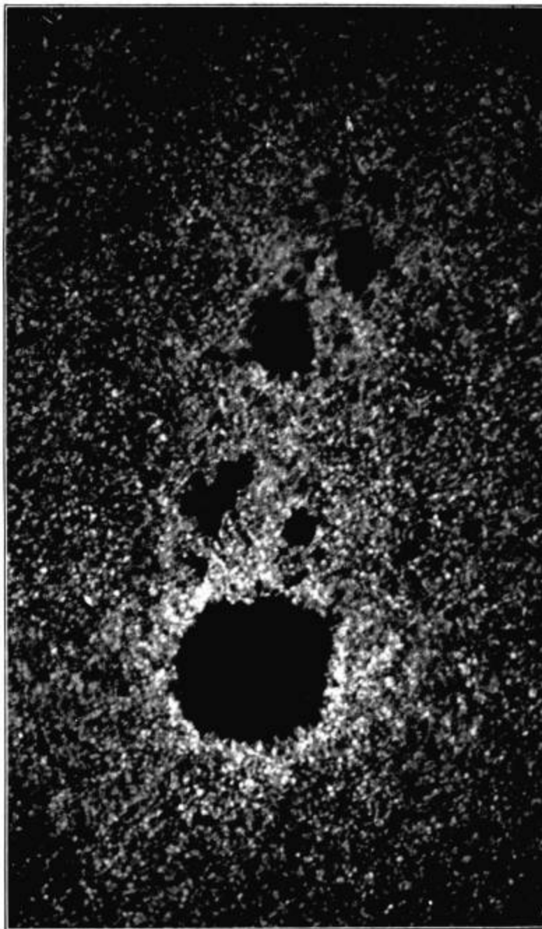
FIG. 96.—A group of sun-spots. From a photograph taken by M. Janssen at Meudon on April 1st, 1894.
