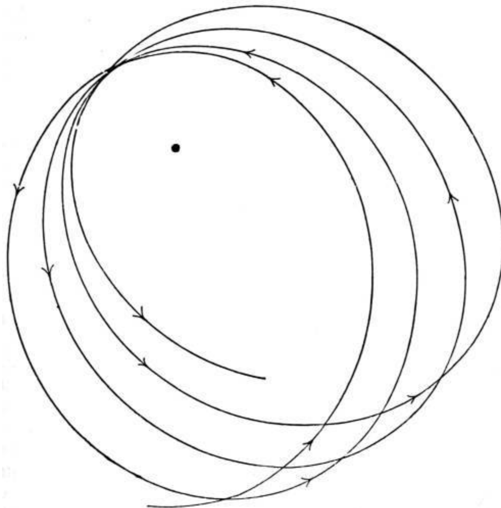
FIG. 81.—A varying ellipse.
