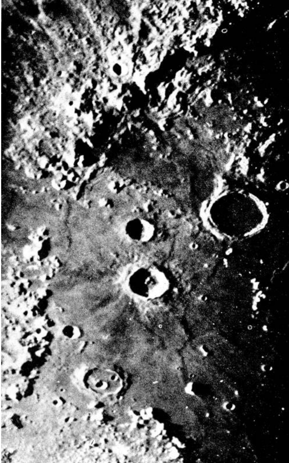
FIG. 94.—The Apennines and adjoining regions of the moon. From a photograph taken at the Paris Observatory.
