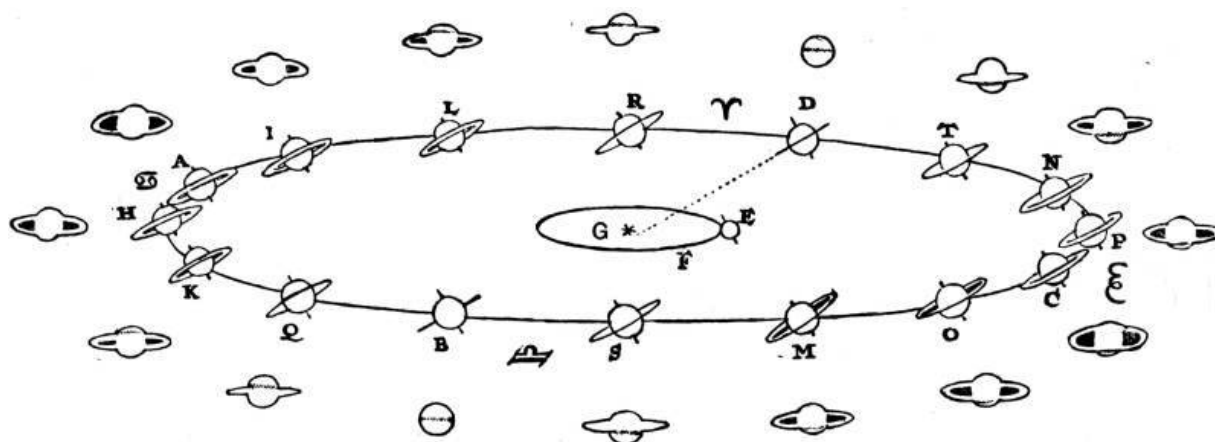
FIG. 66.—The phases of Saturn's ring. From the Systema Saturnium .
