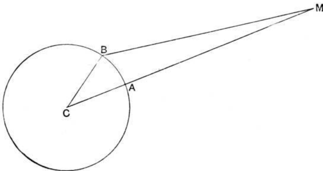
FIG. 31.—Parallax.
