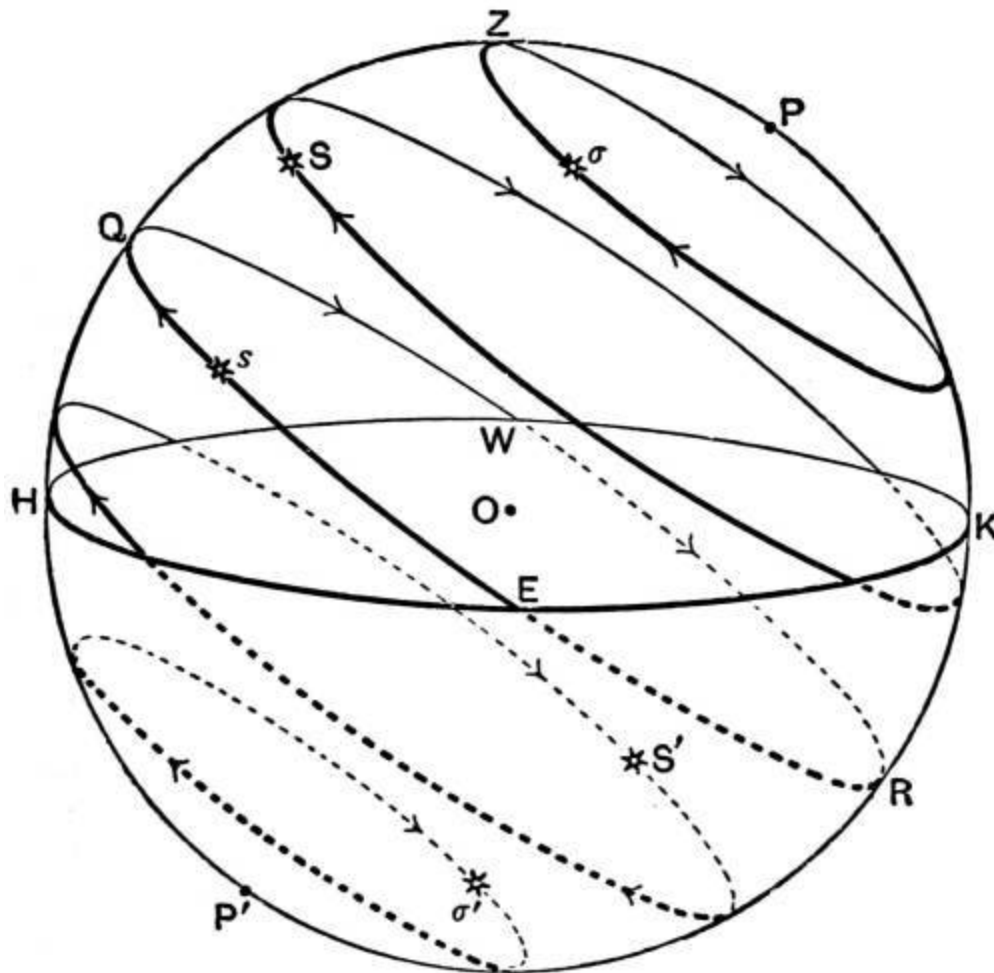
FIG. 3.—The circles of the celestial sphere.
