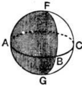
FIG. 9.—The phases of the moon.
