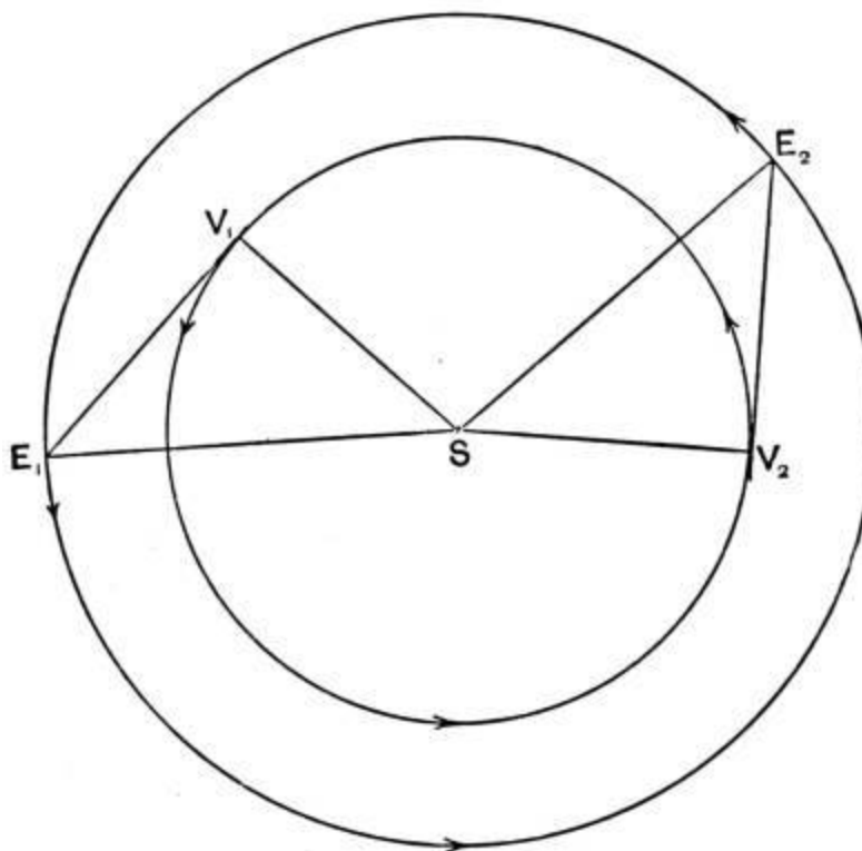
FIG. 44.—The synodic and sidereal periods of Venus.
