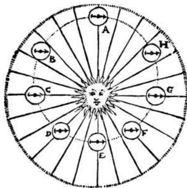
FIG. 63.—Kepler's idea of gravity. From the Epitome .
