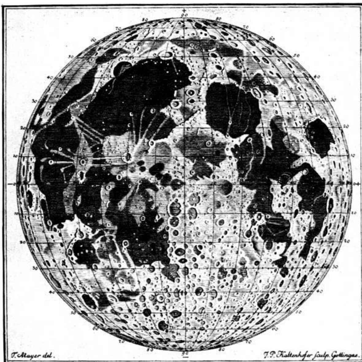
FIG. 79.—Tobias Mayer's map of the moon.
