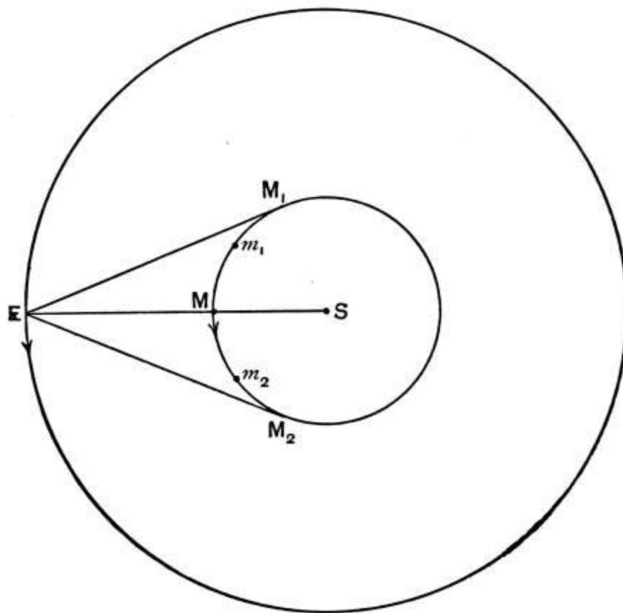
FIG. 47.—The stationary points of Mercury.
