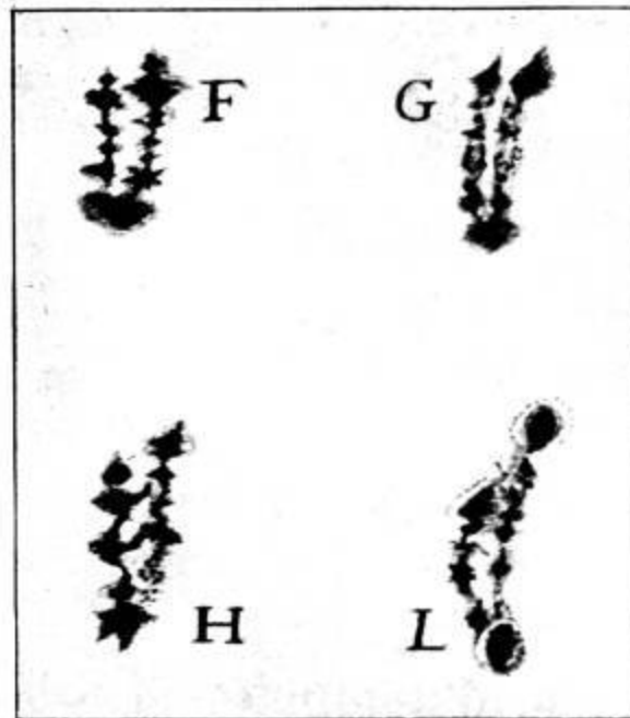
FIG. 55.—Sun-spots. From Galilei's Macchie Solari .
