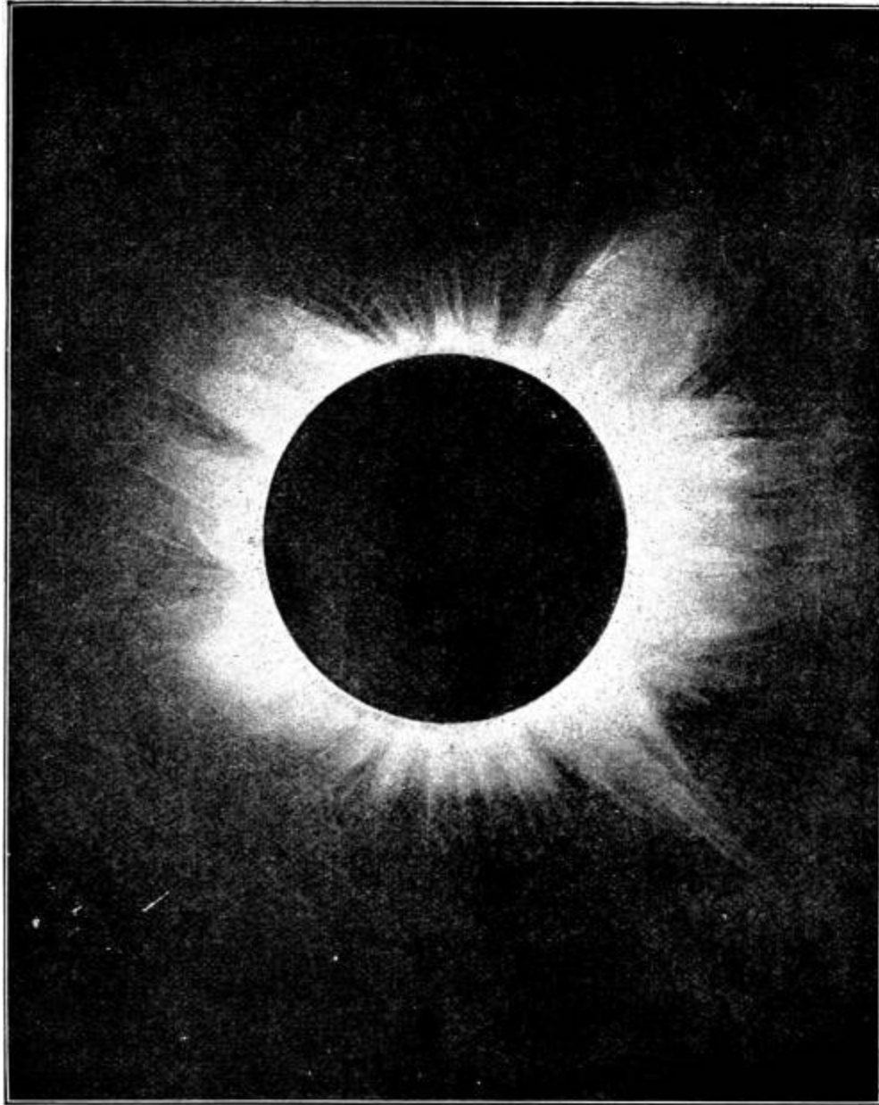
FIG. 98.—The total solar eclipse of August 29th, 1886. From a drawing based on photographs by Dr. Schuster and Mr. Maunder.
