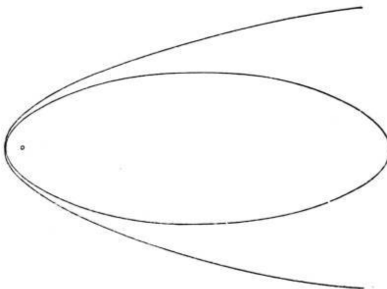
FIG. 73.—An elongated ellipse and a parabola.
