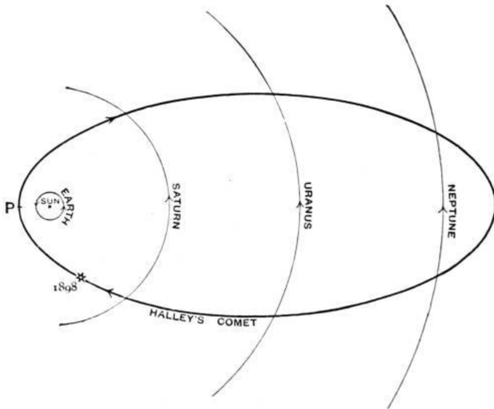
FIG. 80.—The path of Halley's comet.
