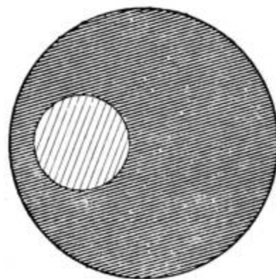
FIG. 29.—Total eclipse of the moon.
