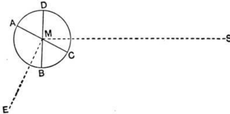
FIG. 8.—The phases of the moon.
