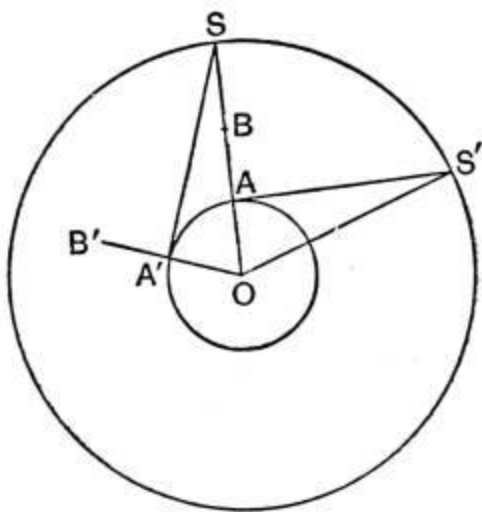
FIG. 39.—The daily rotation of the earth.
