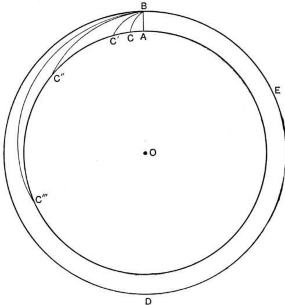
FIG. 71.—The moon as a projectile.
