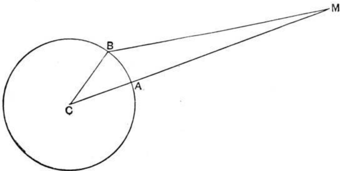
FIG. 33.—Parallax.
