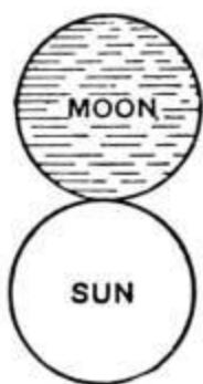
FIG. 27.—The sun and moon.
