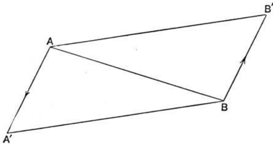
FIG. 37.—Relative motion.
