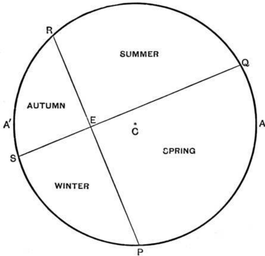
FIG. 18.—The position of the sun's apogee.
