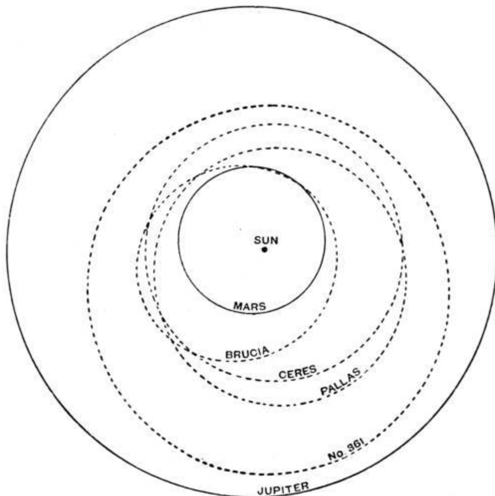
FIG. 89.—Paths of minor planets.
