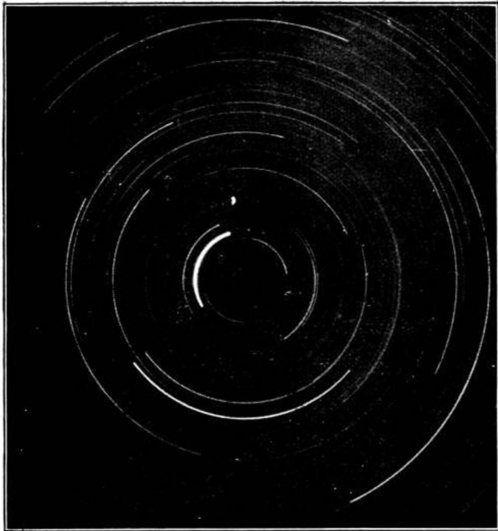
FIG. 2.—The paths of circumpolar stars, shewing their movement during seven hours. From a photograph by Mr. H. Pain. The thickest line is the path of the pole star.
