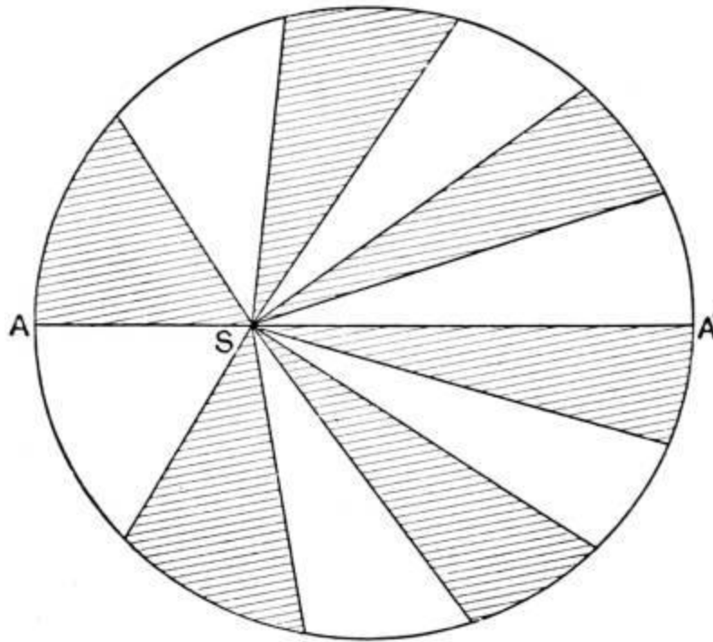
FIG. 60.—Kepler's second law.
