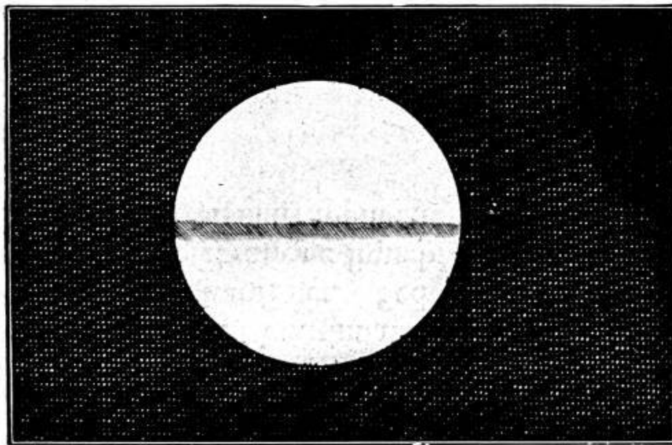
FIG. 65.—Saturn, with the ring seen edge-wise. From the Systema Saturnium .
