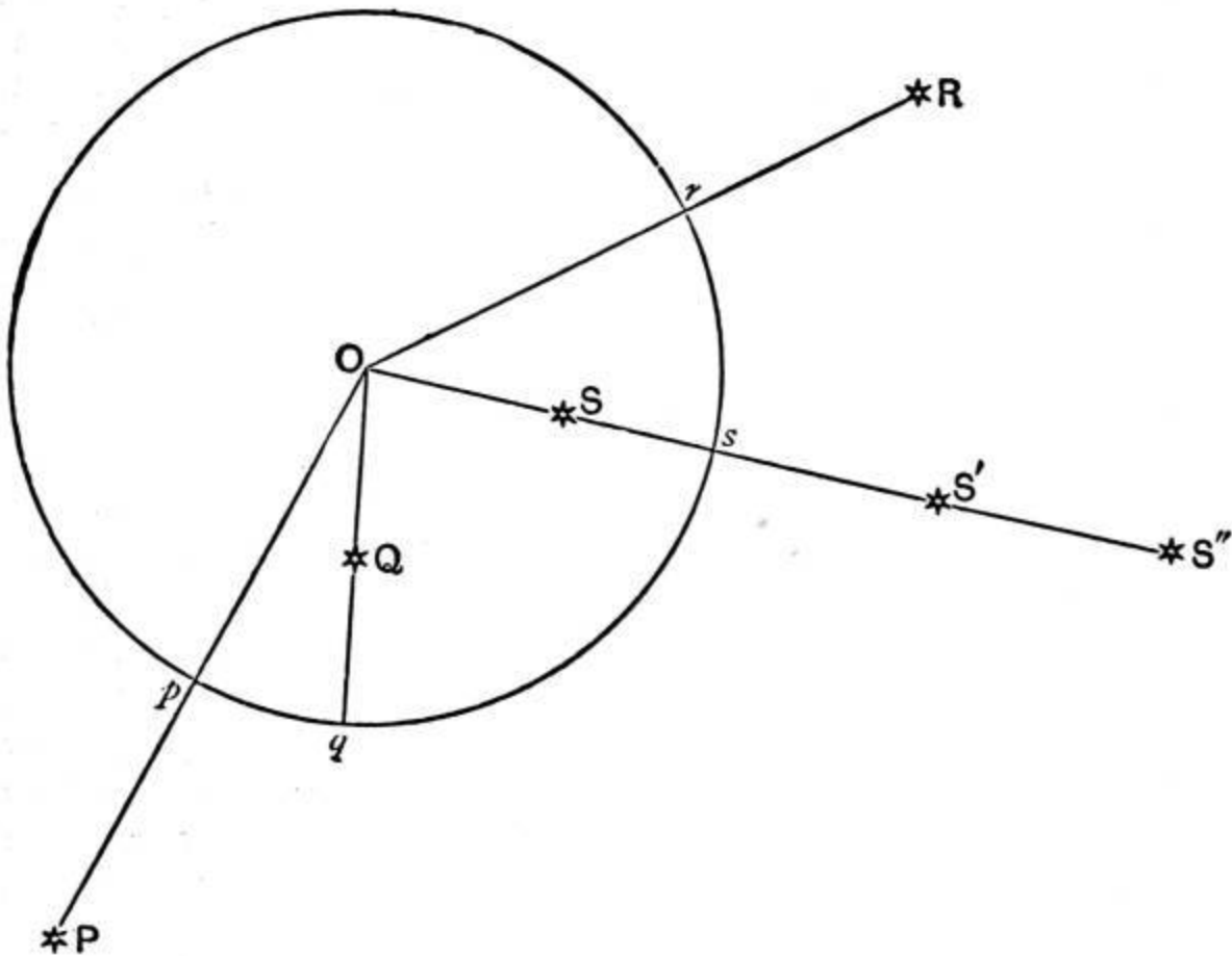
FIG. 1.—The celestial sphere.
