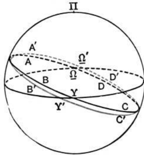
FIG. 33.—The precession of the equinoxes.
