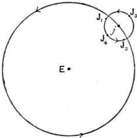
FIG. 34.—Jupiter's epicycle and deferent.
