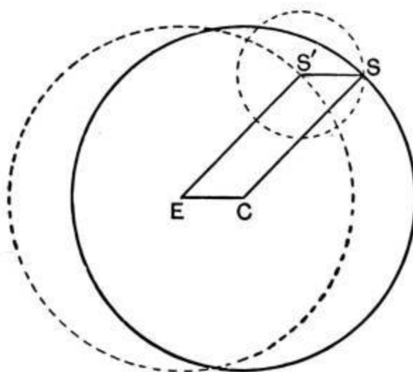
FIG. 19.—The epicycle and the deferent.
