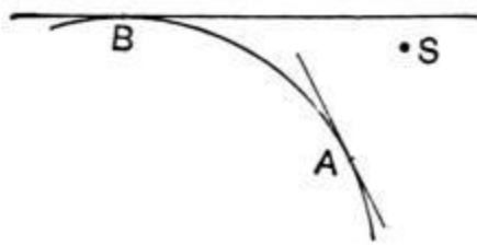
FIG. 12.—The curvature of the earth.
