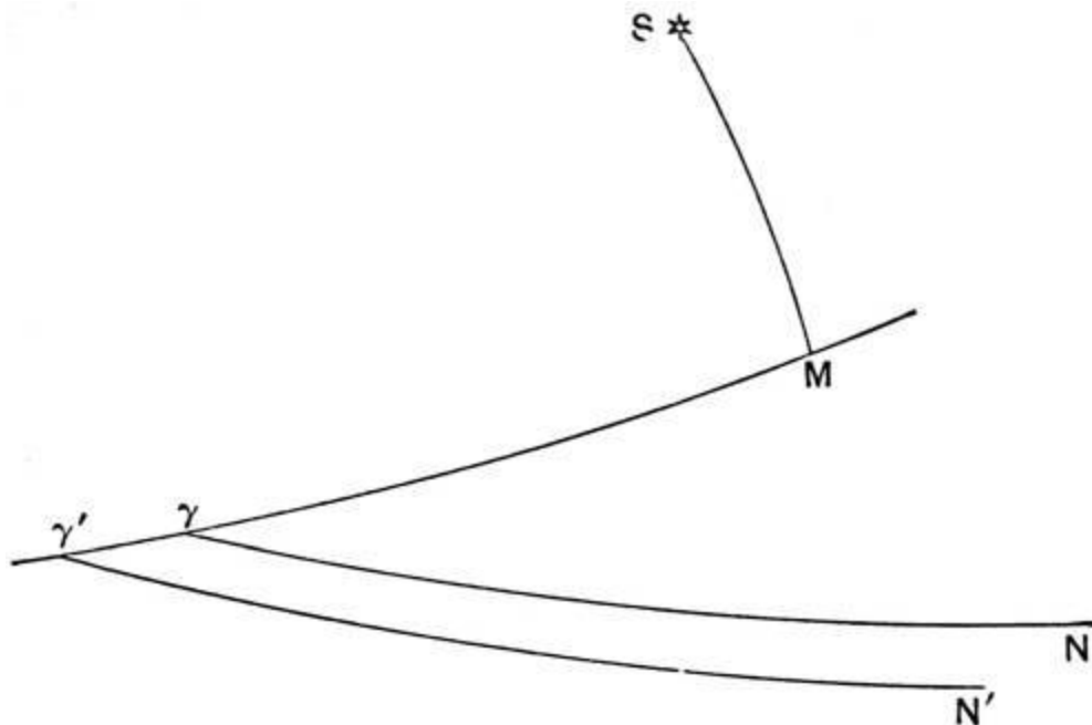
FIG. 22.—The movement of the equator.
