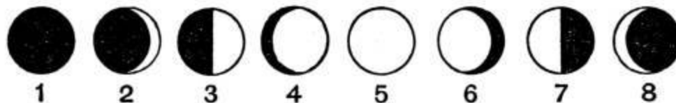
FIG. 11.—The phases of the moon.
