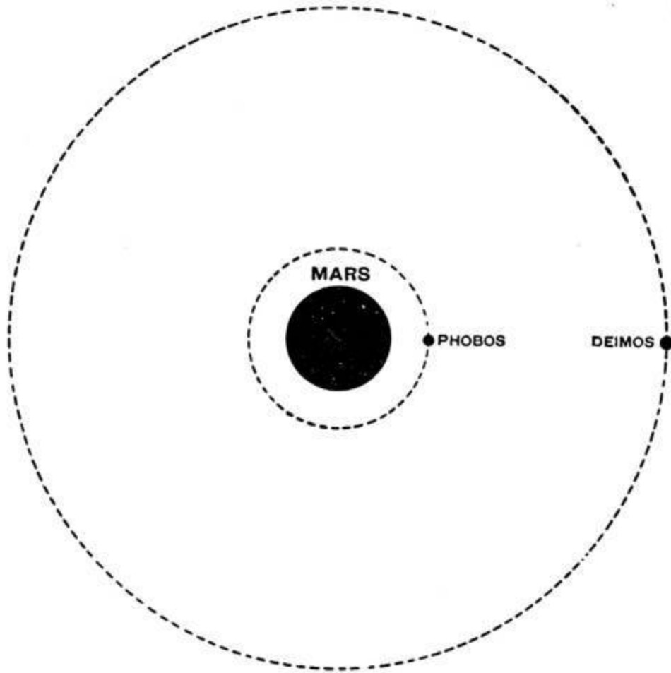
FIG. 92.—Mars and its satellites.
