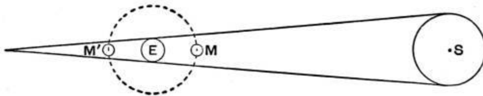
FIG. 25.—The earth's shadow.
