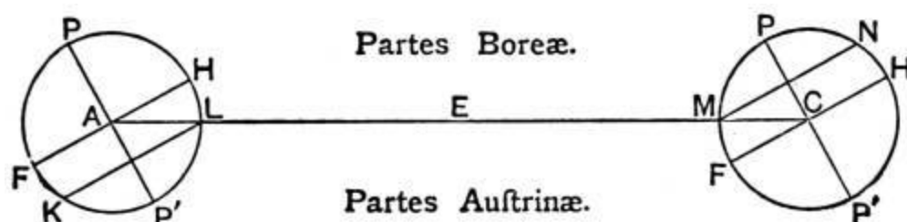
FIG. 42.—Copernican explanation of the seasons. From the De Revolutionibus .
