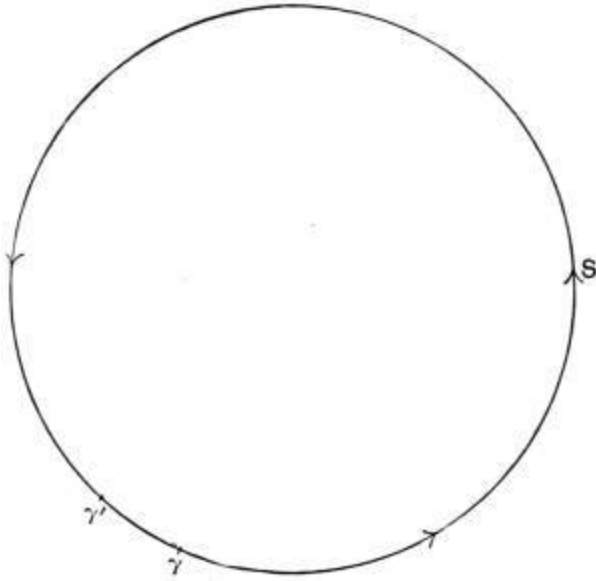
FIG. 24.—The precession of the equinoxes.
