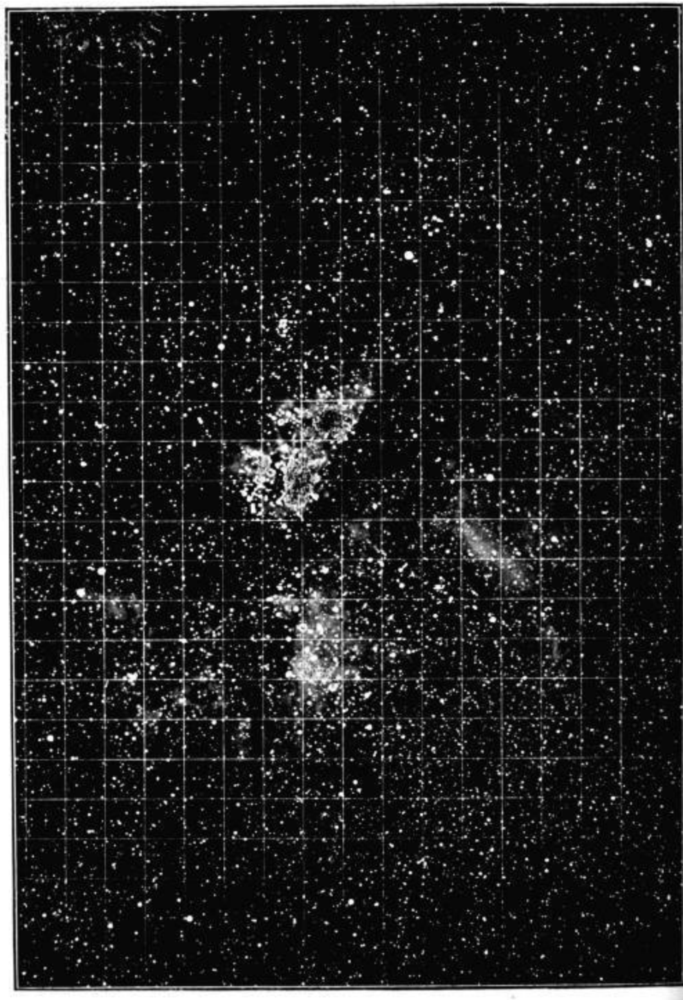
FIG. 100.—The nebula about \eta Argus.
