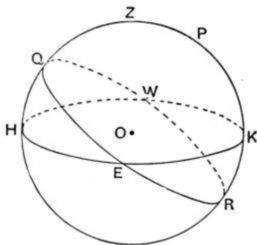
FIG. 15.—The equator, the horizon, and the meridian.
