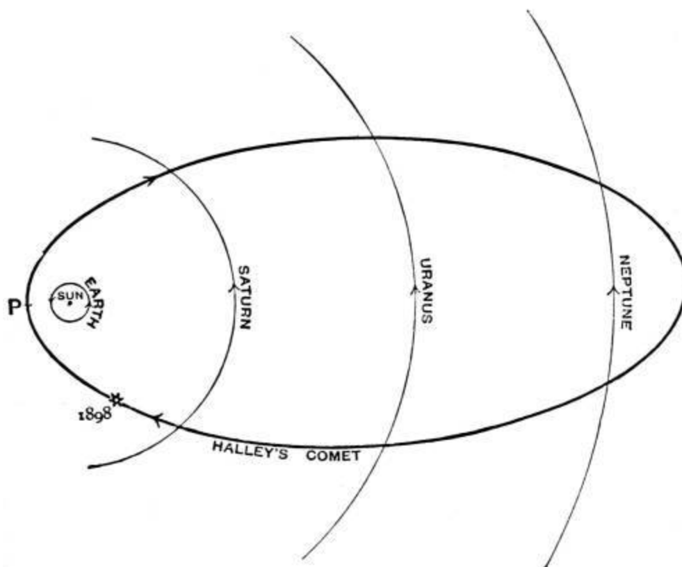
FIG. 87.—The path of Halley's comet.
