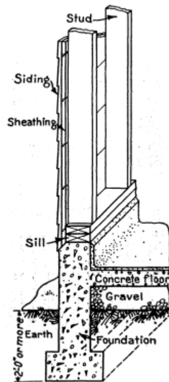
FIGURE 3.—Foundation and floor suitable for most types of farm buildings
