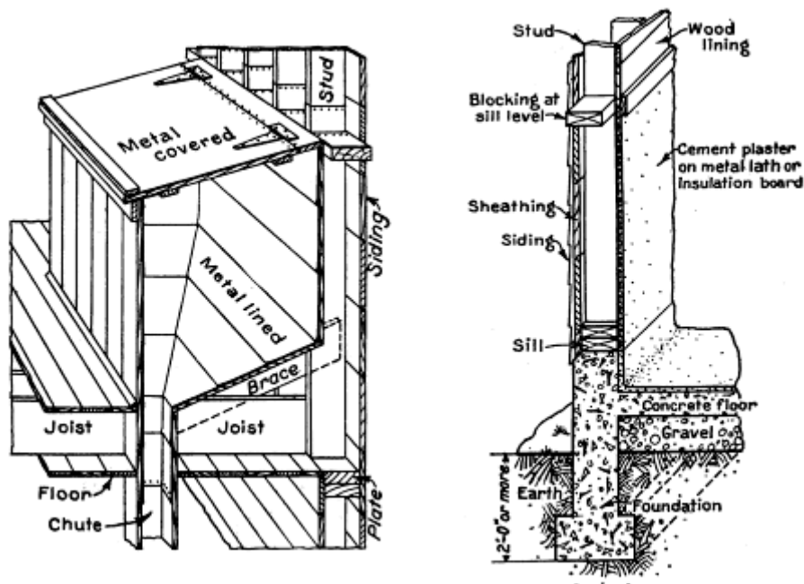
FIGURE 6.—A convenient upper-story rat-proof grain bin
