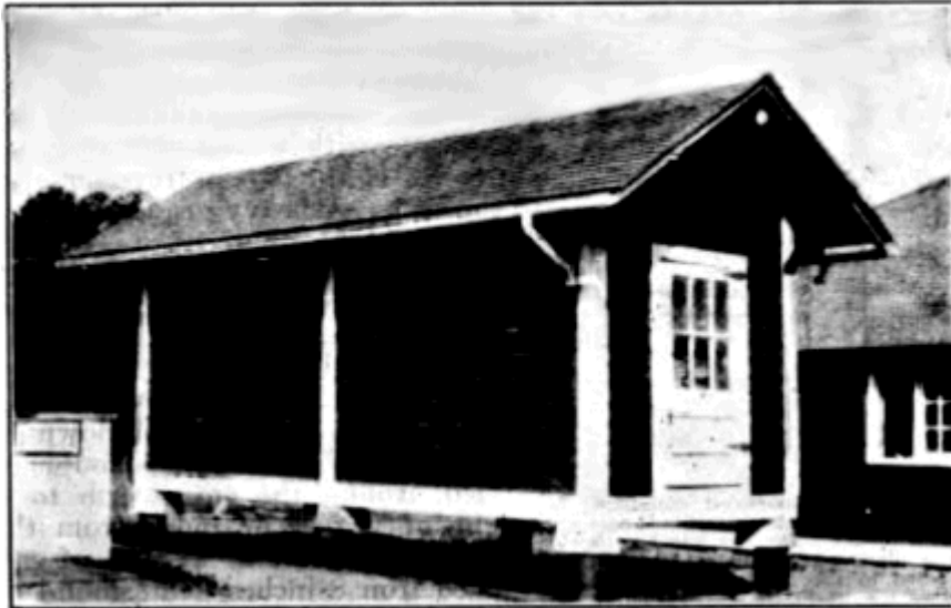
FIGURE 9.—An inexpensive method of rat proofing a corner crib. It is supported by glazed tiles capped with galvanized washtubs, which, though not attractive in appearance, have successfully kept out rats
