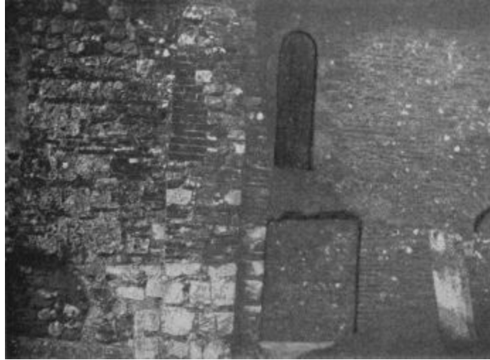
FIG. 7. Portion of chancel wall, south side, St Martin's Church, Canterbury. Roman tiles are seen abundantly in the wall on the right, and in the round arch; they are also bonded into the wall on the left. The wall is mainly seventh-century work, but the round-headed doorway is later, and the buttress has been modernized. The flat-headed doorway is probably original.
