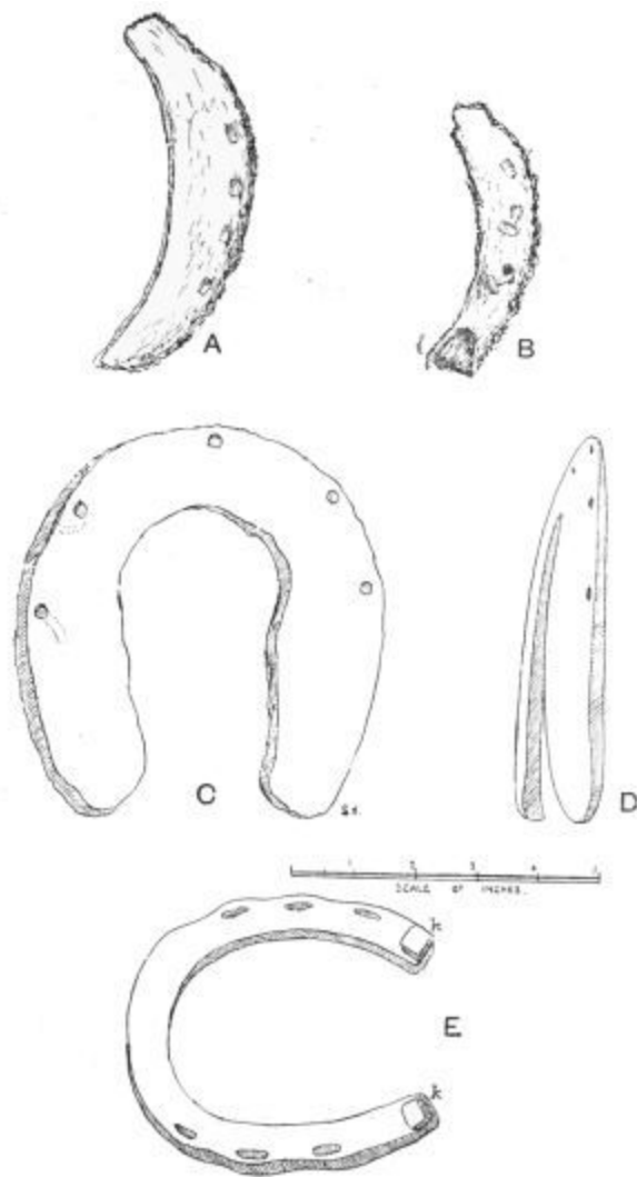
FIG. 83. A, B. Portions of small horseshoes, much corroded, found by Pitt-Rivers in Cranborne Chase. The worn fragment, B, exhibits three holes, with T-shaped nails. There is a calkin at k , formed by turning up the lower surface of the shoe. C. Ancient horseshoe found by Mr E. C. Youens, at Edenbridge, Kent. The shoe, which is formed of wrought iron, is markedly concavo-convex, the convex surface being the lower one. The "wale-holes" are very near the edge. There is no raised rim. D. Side view of the same shoe. E. Small horseshoe, Guildhall Museum, London. Roman layer, City. The curve is sinuous, the holes are elliptical, and the calkins are well formed.
