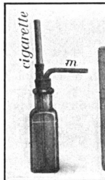
Experiment (by Davison) to show how the nicotine in six cigarettes was sufficient to kill this fish. The smoke from the cigarettes was passed through the water in which the fish is swimming.
