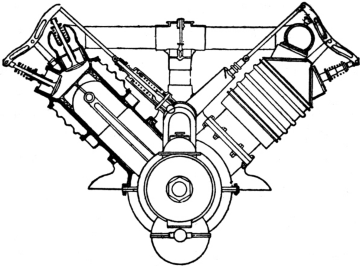
Dorman 80 horse-power Vee-type Engine.
