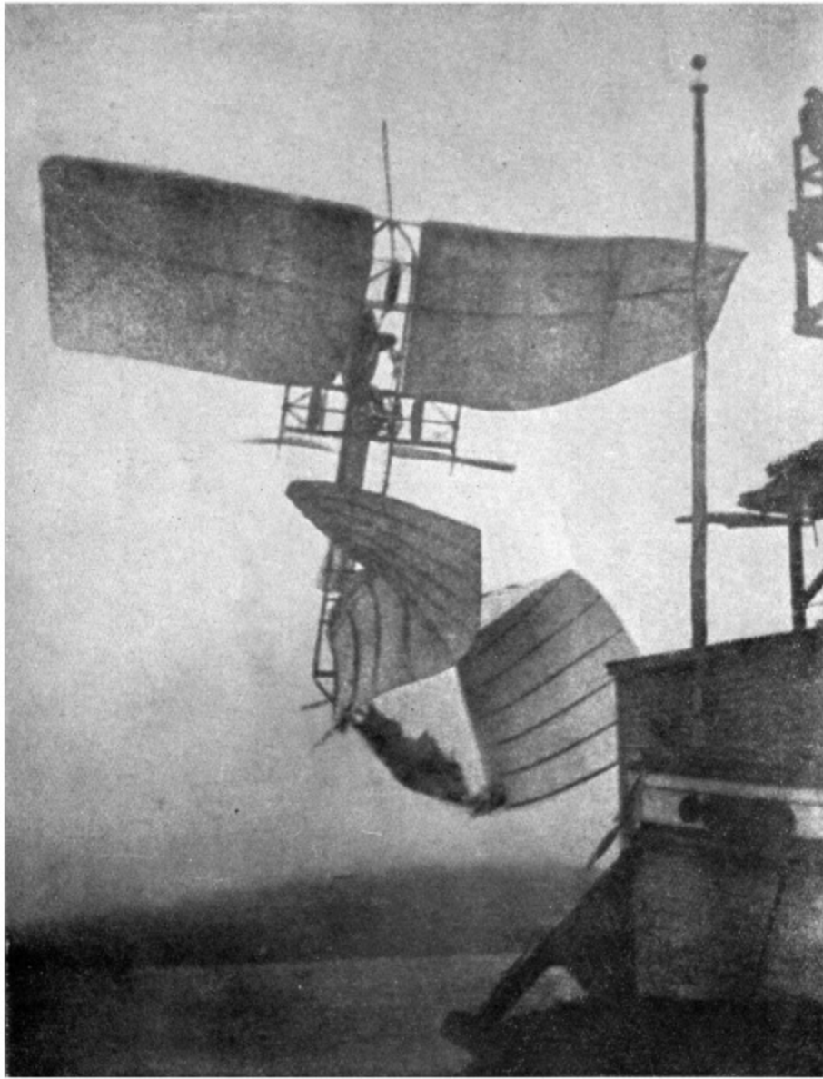
Trial of full-size Langley Aerodrome, 8th December, 1903.
