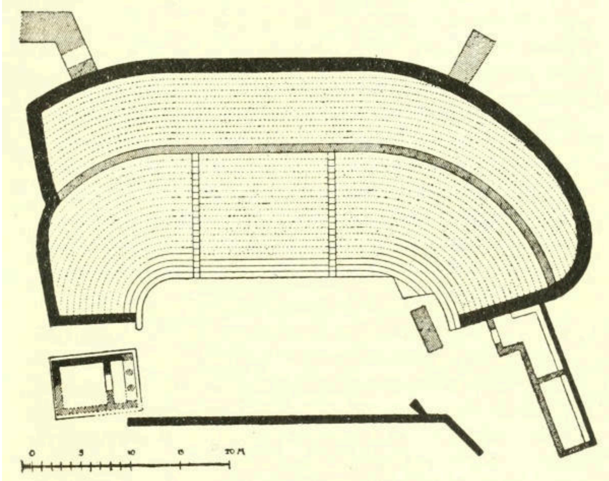
FIG. 70.—Ground Plan of the Theater at Thoricus in Attica
