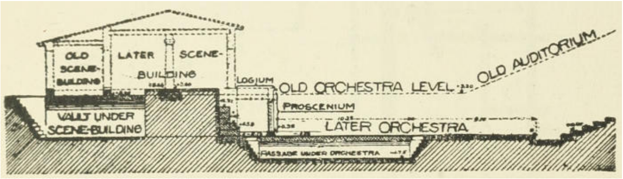
FIG. 54.—Cross-Section of the Theater at Eretria
