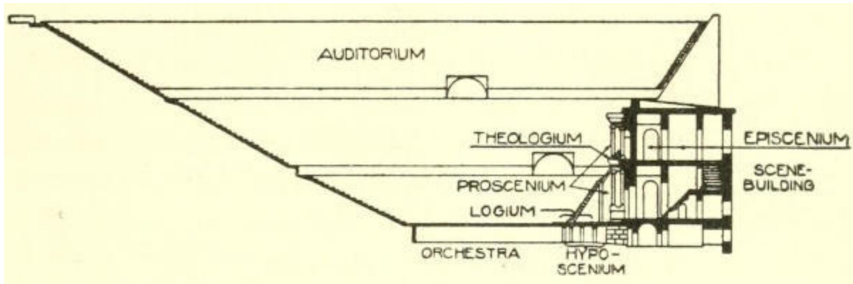
FIG. 24.—Cross-Section of the Graeco-Roman Theater at Ephesus with Names of Its Parts.
