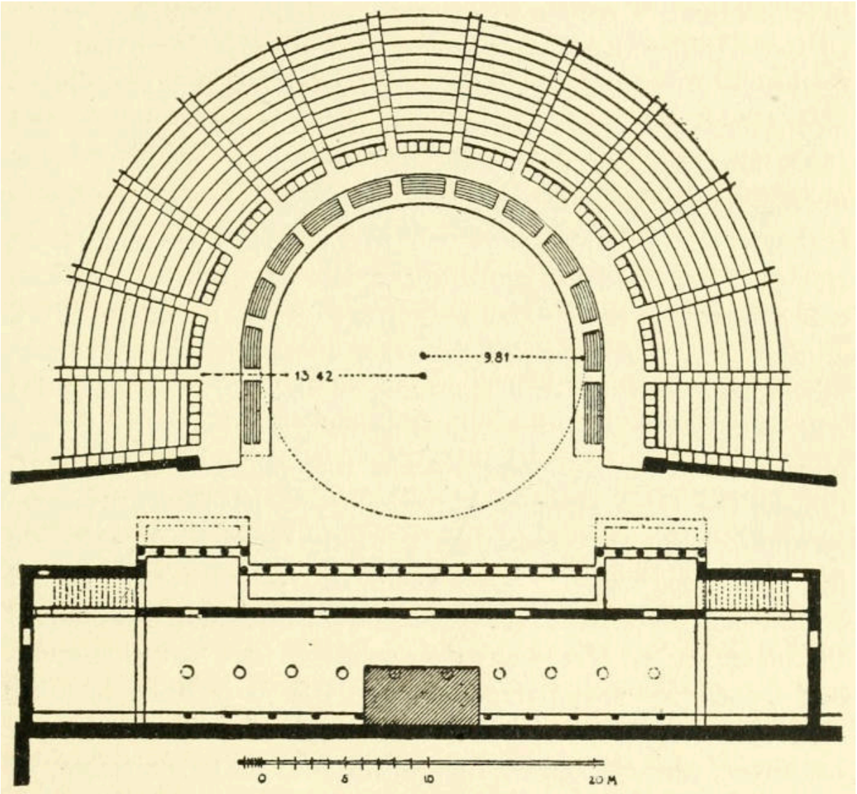
FIG. 38.—Ground Plan of the Hellenistic Theater in Athens According to Dörpfeld.
