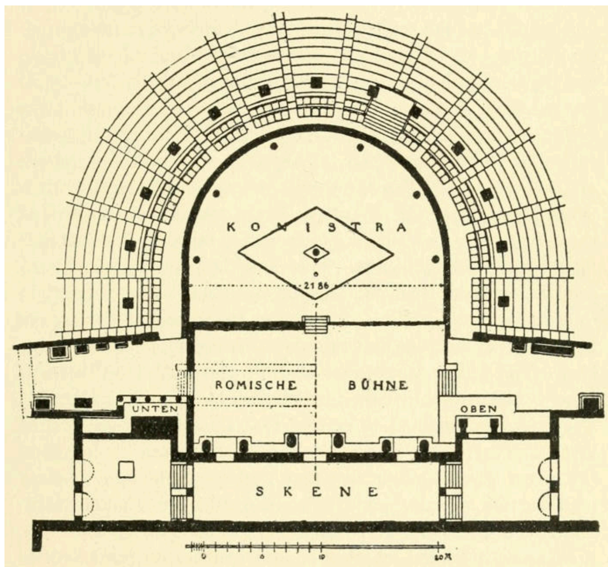
FIG. 40.—Plan of the Romanized Theater in Athens According to Dörpfeld
