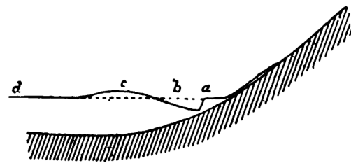
FIG. 73.—Displacement of alluvium at foot of a hill.
