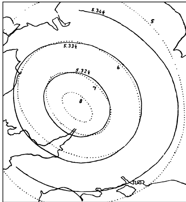
FIG. 62.—Coseismic lines of the Hereford earthquake. ( Davison. ) ToList
