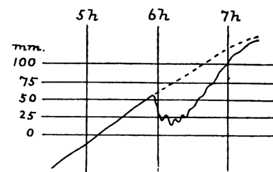
FIG. 38.—Record of tide-gauge at Nice. ( Issel. ) ToList
