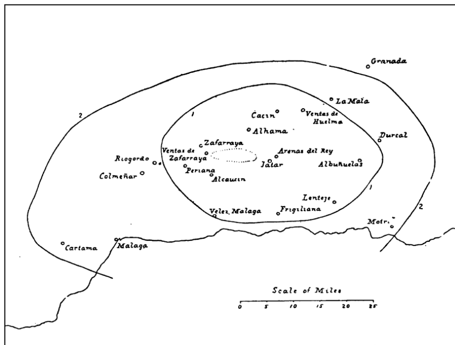
FIG. 19.—Iseismal lines of Andalusian earthquake. ( Taramelli and Mercalli. ) ToList
