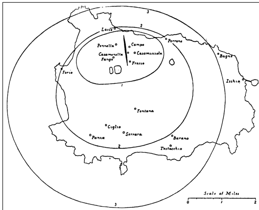
FIG. 16.—Iseismal lines of the Ischian earthquake of 1883. To List
