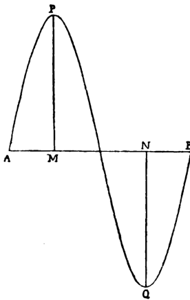
FIG. 1.—Diagram to illustrate simple harmonic motion. To List
