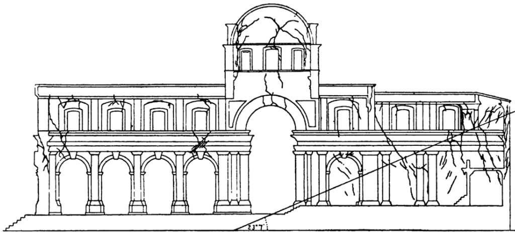
FIG. 12.—Vertical section of Cathedral Church at Potenza.
