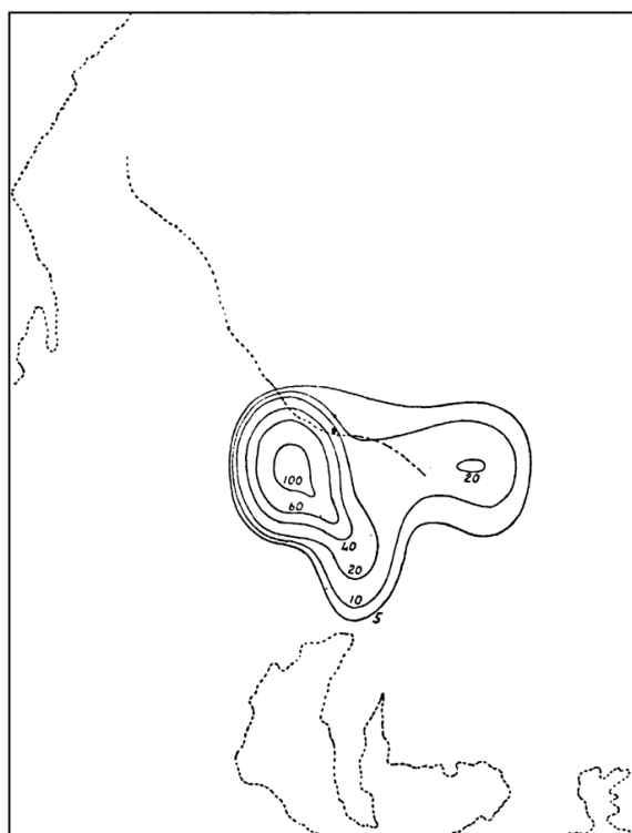
FIG. 56.—Distribution of After-shocks in Space (March-April). ( Davison. ) ToList
