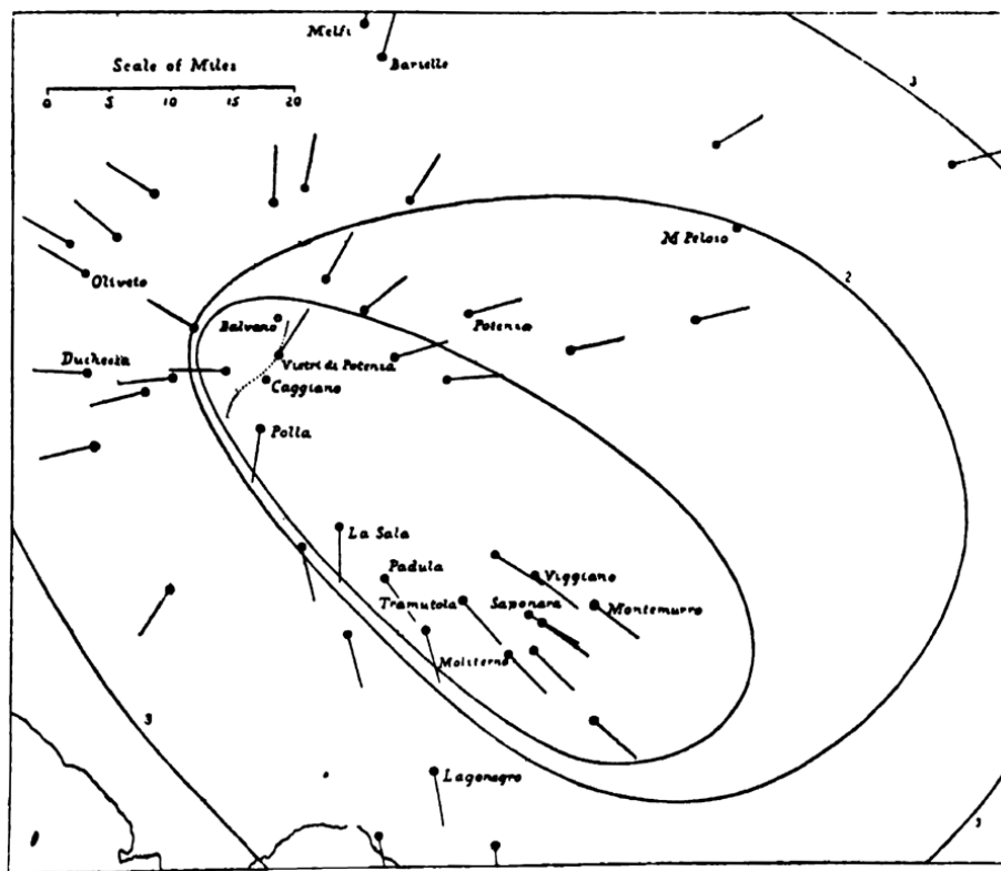
FIG. 9.—Meizoseismal area of Neapolitan earthquake. (Mallet.) ToList
