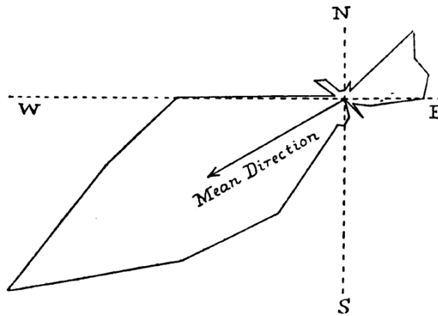
FIG. 43.—Plan of Directions of Fall of Overturned Bodies at Nagoya. ToList
