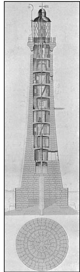
SECTIONS OF THE EDDYSTONE LIGHTHOUSE,
