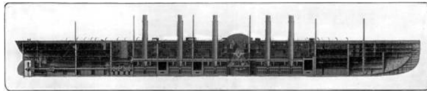
SECTION OF THE "GREAT EASTERN," THE LARGEST SHIP EVER BUILT.
