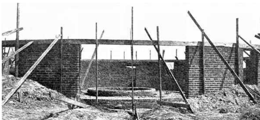
FIG. 12. FIRST STORY WALL, AND FOUNDATION FOR SILO, FEED ALLEY, AND MANGER; SILL IN PLACE, READY FOR JOISTS AND STUDS.
