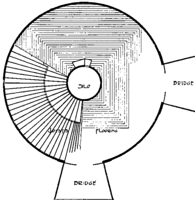
FIG. 17. SHOWING ARRANGEMENT OF JOISTS AND HOW THE FLOOR IS LAID.
