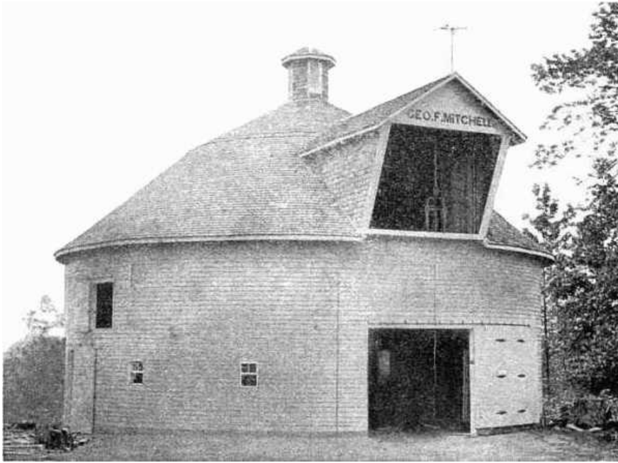
FIG. 38. BARN 48 FEET IN DIAMETER, 16-FOOT POSTS; NOTE METHOD OF TAKING HAY INTO SMALL ROUND BARN.
