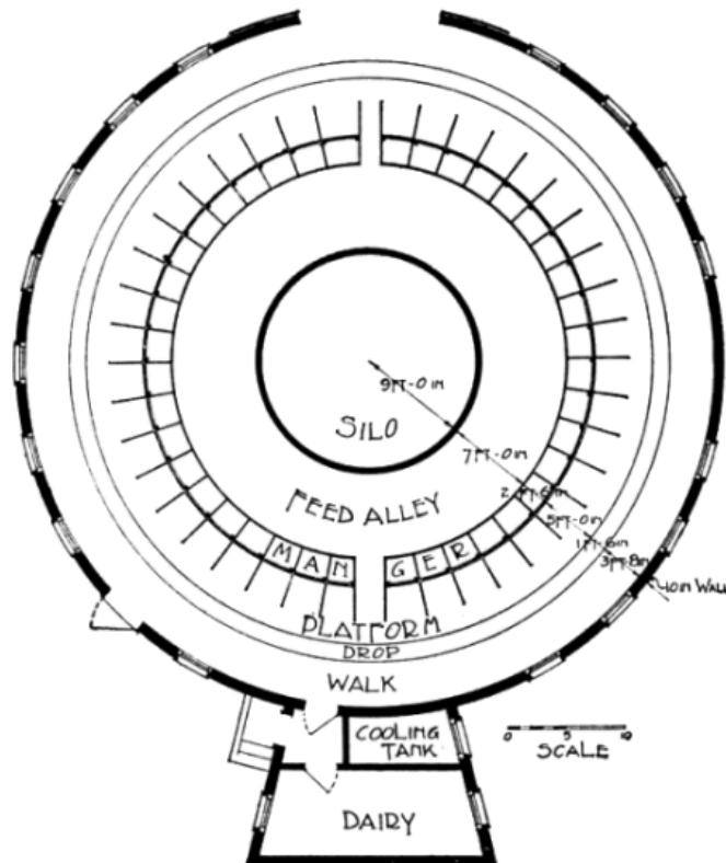
FIG. 25. SHOWING HOW THIS 60-FOOT BARN MAY BE ARRANGED TO ACCOMMODATE 40 COWS IN STALLS. TO SUPPLY THIS SIZED HERD AND THE NECESSARY YOUNG STOCK WITH SILAGE FOR EIGHT MONTHS WOULD REQUIRE A 370-TON SILO, OR ONE 18 FEET IN DIAMETER AND 56 FEET DEEP; WITH A SEVEN-FOOT FEED ALLEY AND A 2½-FOOT MANGER, THE CIRCLE AT THE STANCHIONS WOULD BE 38 FEET IN DIAMETER, OR 119⅓ FEET IN CIRCUMFERENCE; ALLOWING 4¼ FEET FOR TWO PASSAGE WAYS, THE STALLS WOULD BE 2 FEET 10-1/2 INCHES WIDE AT THE STANCHION, AND 3 FEET 6 INCHES AT THE DROP.
