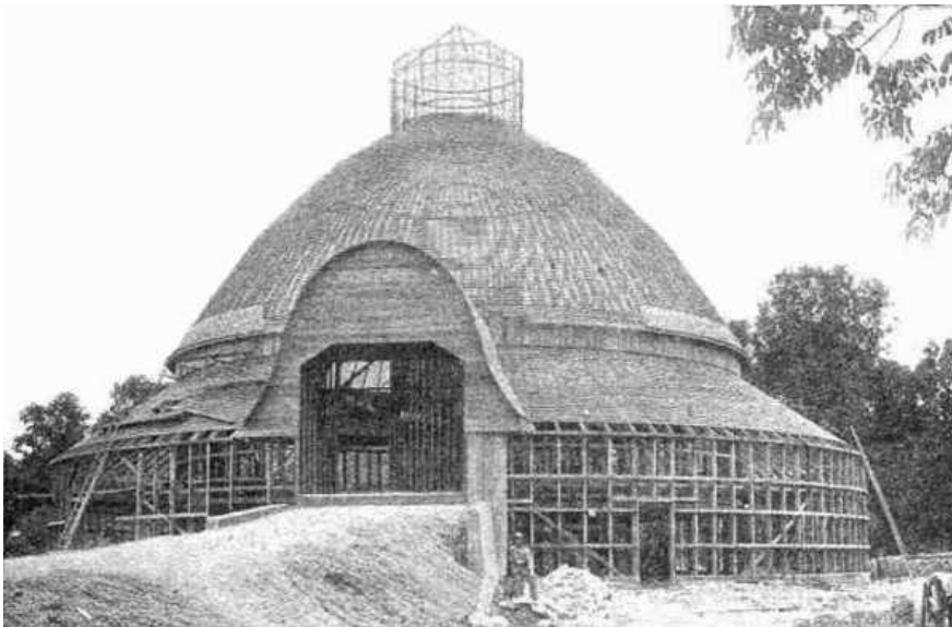
FIG. 39. SHOWING CONSTRUCTION OF BARN IN FIG. 40 . HOOPS IN PLACE READY FOR PERPENDICULAR SIDING; ROOF SHEATHED FOR SHINGLES.
