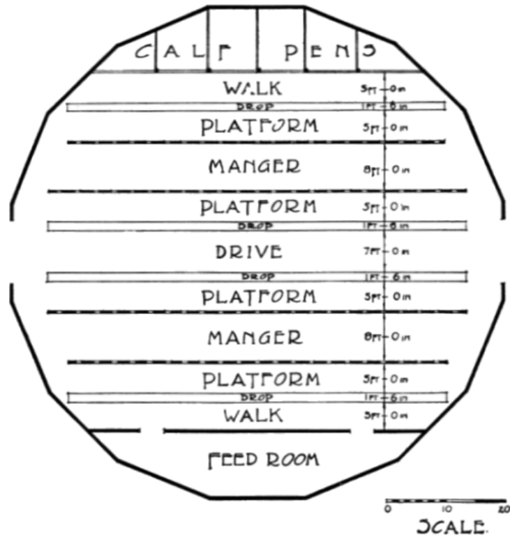
FIG. 42. ARRANGEMENT OF COW STABLE IN BARN NO. 6.
