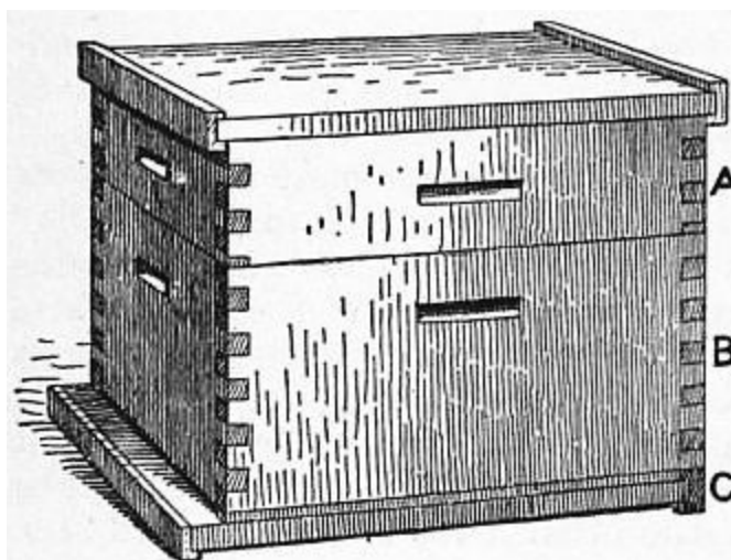
FIG. 15.—Langstroth Hive.
