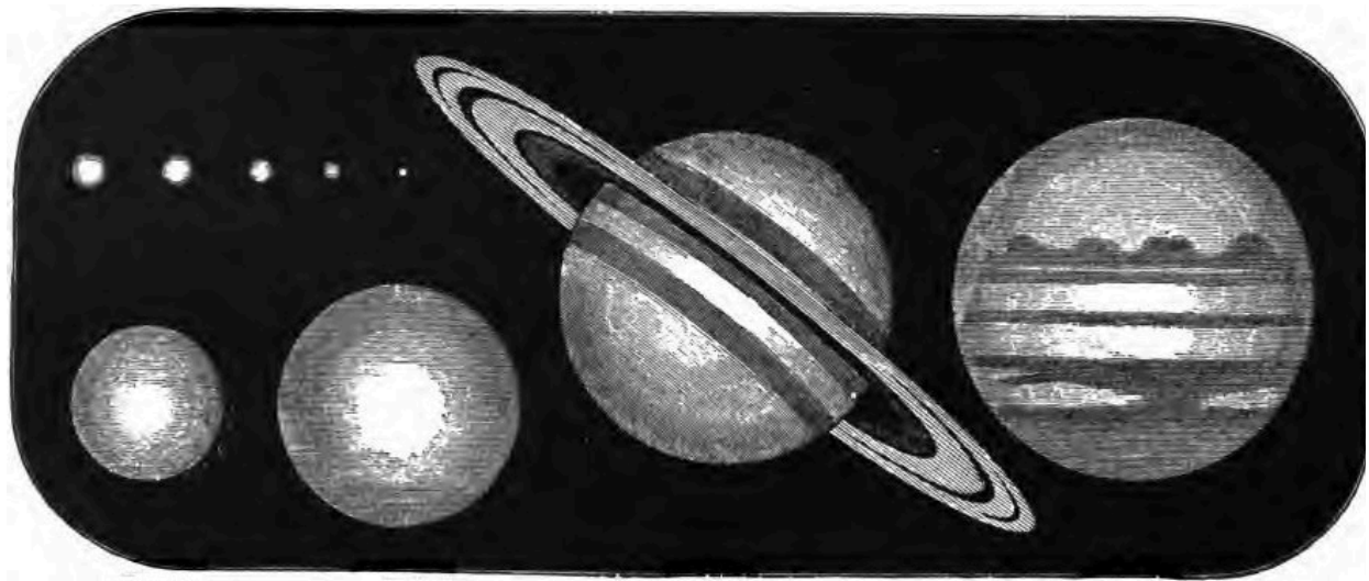
Comparative Size of Planets
