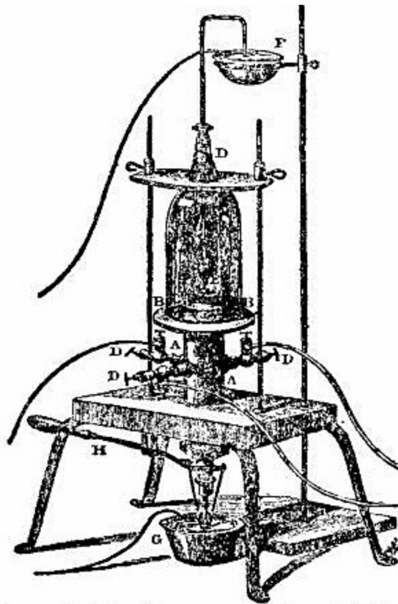
The first American electric furnace, constructed by Robert Hare of Philadelphia. From "Chemistry in America," by Edgar Fahs Smith
