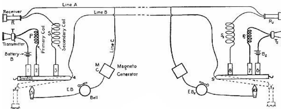
FIG. 64.—A diagrammatic representation of a telephonic circuit.
