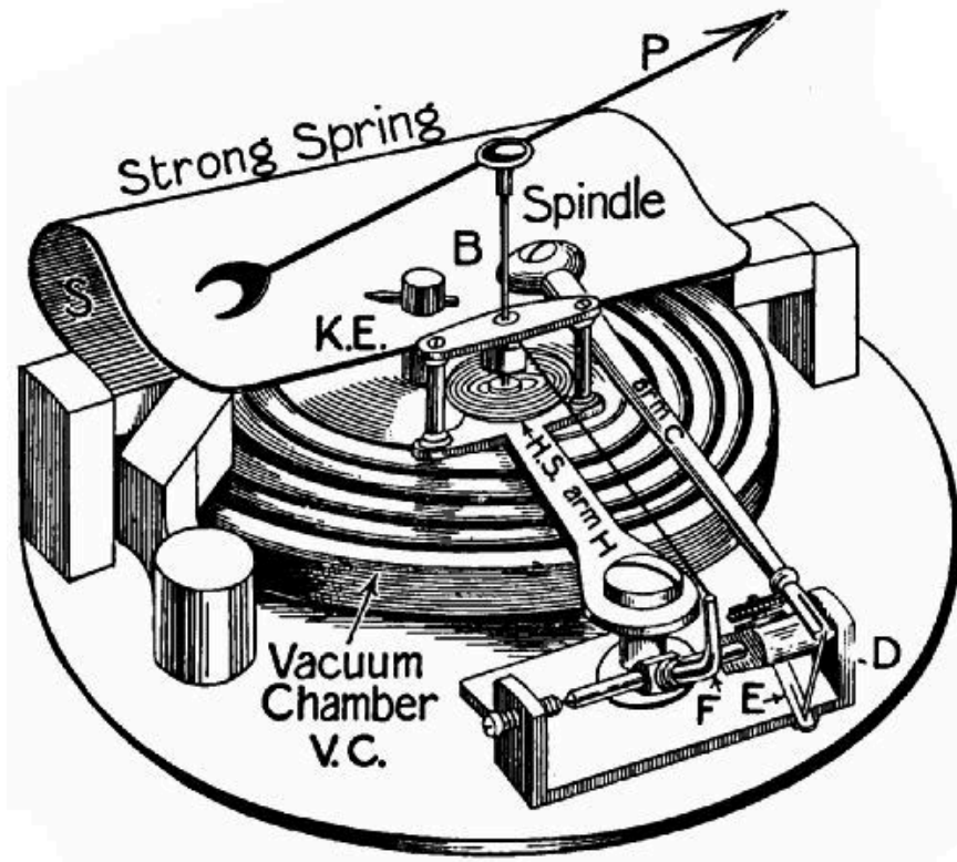
FIG. 155.—An aneroid barometer.
