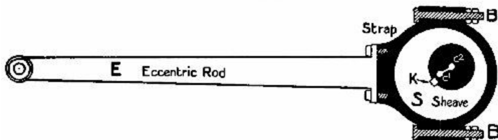
FIG. 23.—The eccentric and its rod.
