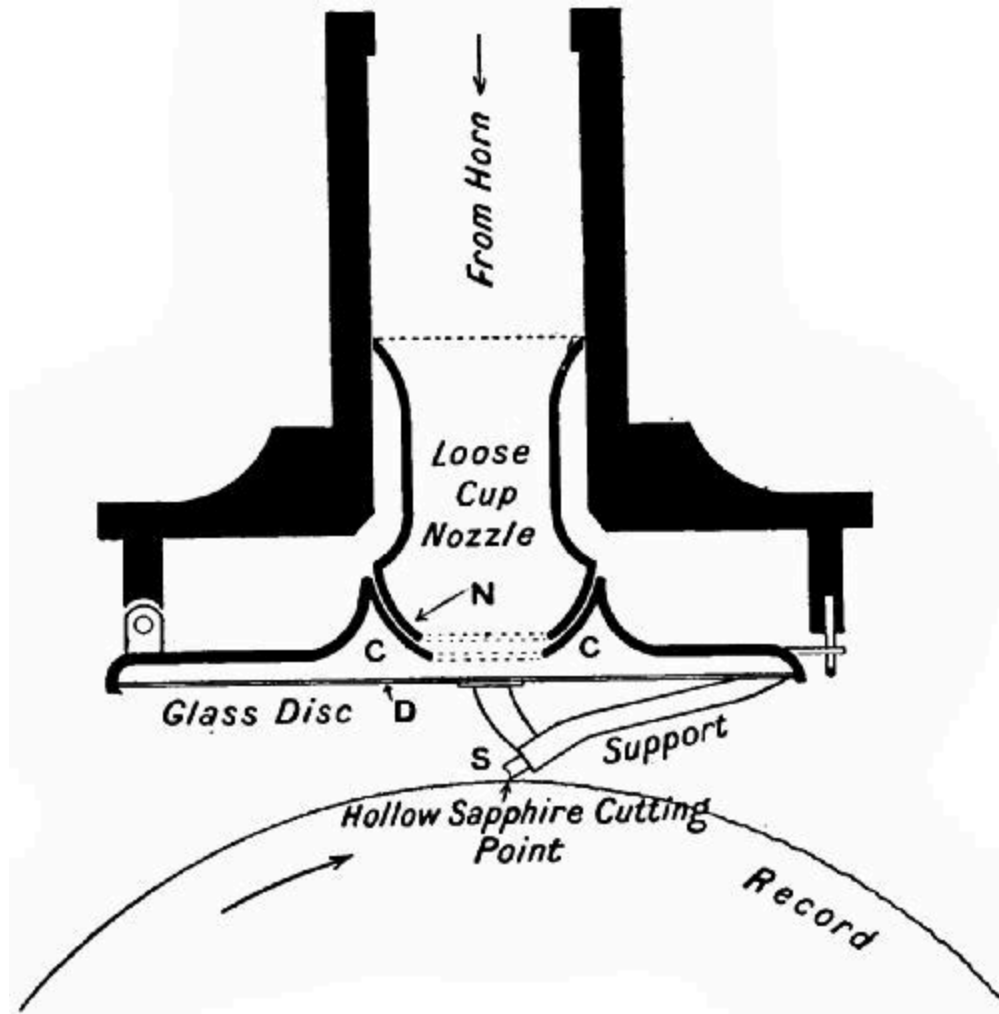
FIG. 147.—Section of an Edison Bell phonograph recorder.
