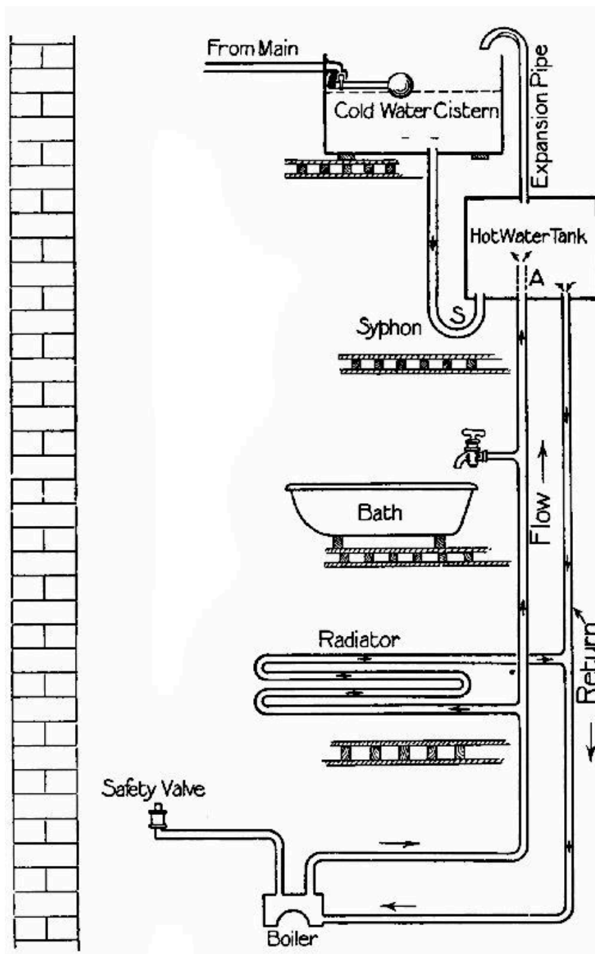
FIG. 192.—The "tank" system of hot-water supply.
