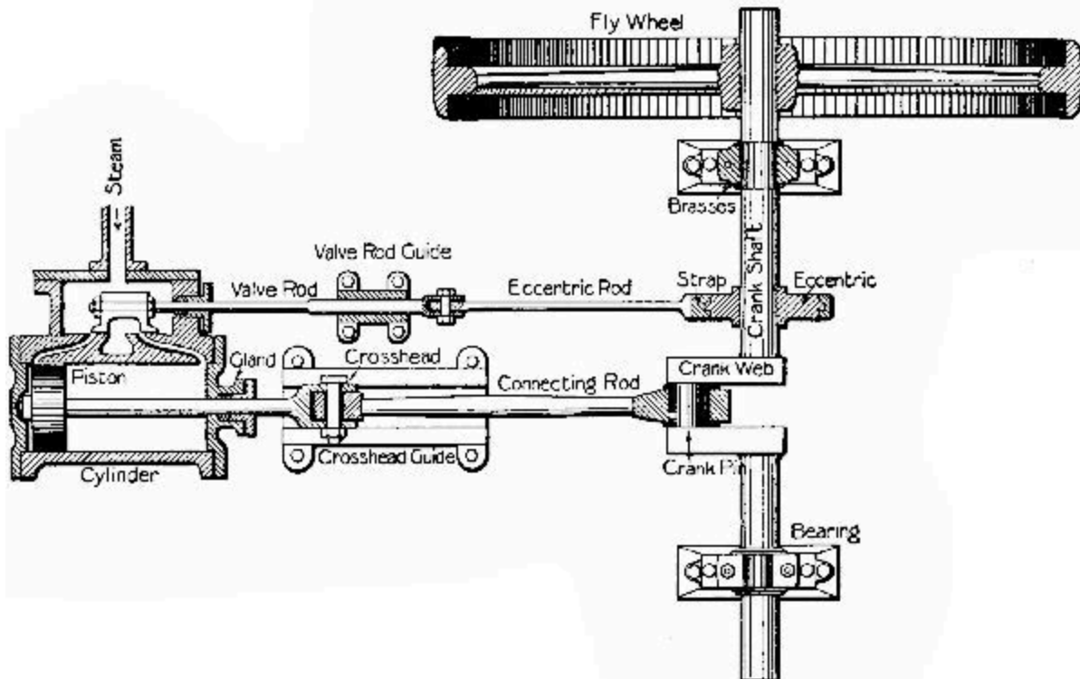
FIG. 18.—Sectional plan of a horizontal engine.
