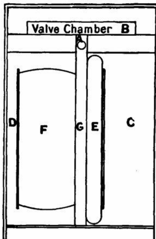
FIG. 200.—Sketch of the bellows and chambers of a "dry" gas meter.
