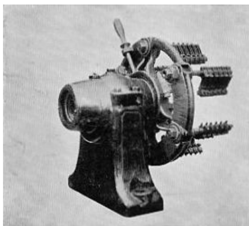
FIG. 76.—The brushes of a Holmes dynamo.
