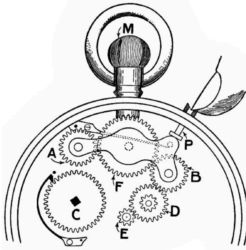
FIG. 210.—The hand-setting mechanism in action.
