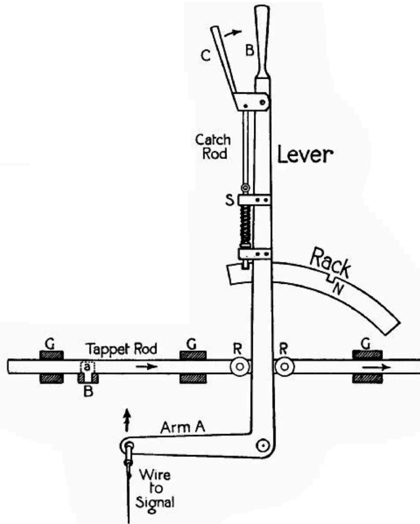
FIG. 93.—A signal lever and its connections. To move the lever, c is pressed towards B raising the catch-rod from its nick in the rack, G G G , guides; R R , anti-friction rollers; s , sockets for catch-rod to work in.
