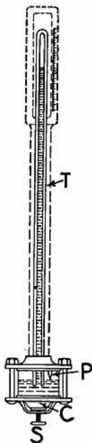
FIG. 152.—A Fortin barometer.
