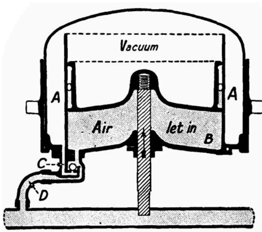
FIG. 86.—Vacuum brake "on."
