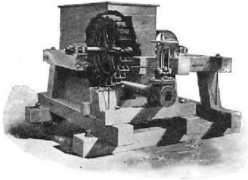
FIG. 188.—Pelton wheel mounted, with nozzle in position.
