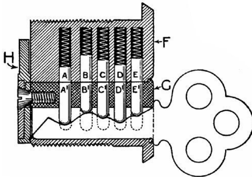
FIG. 219.—Section of a Yale lock.
