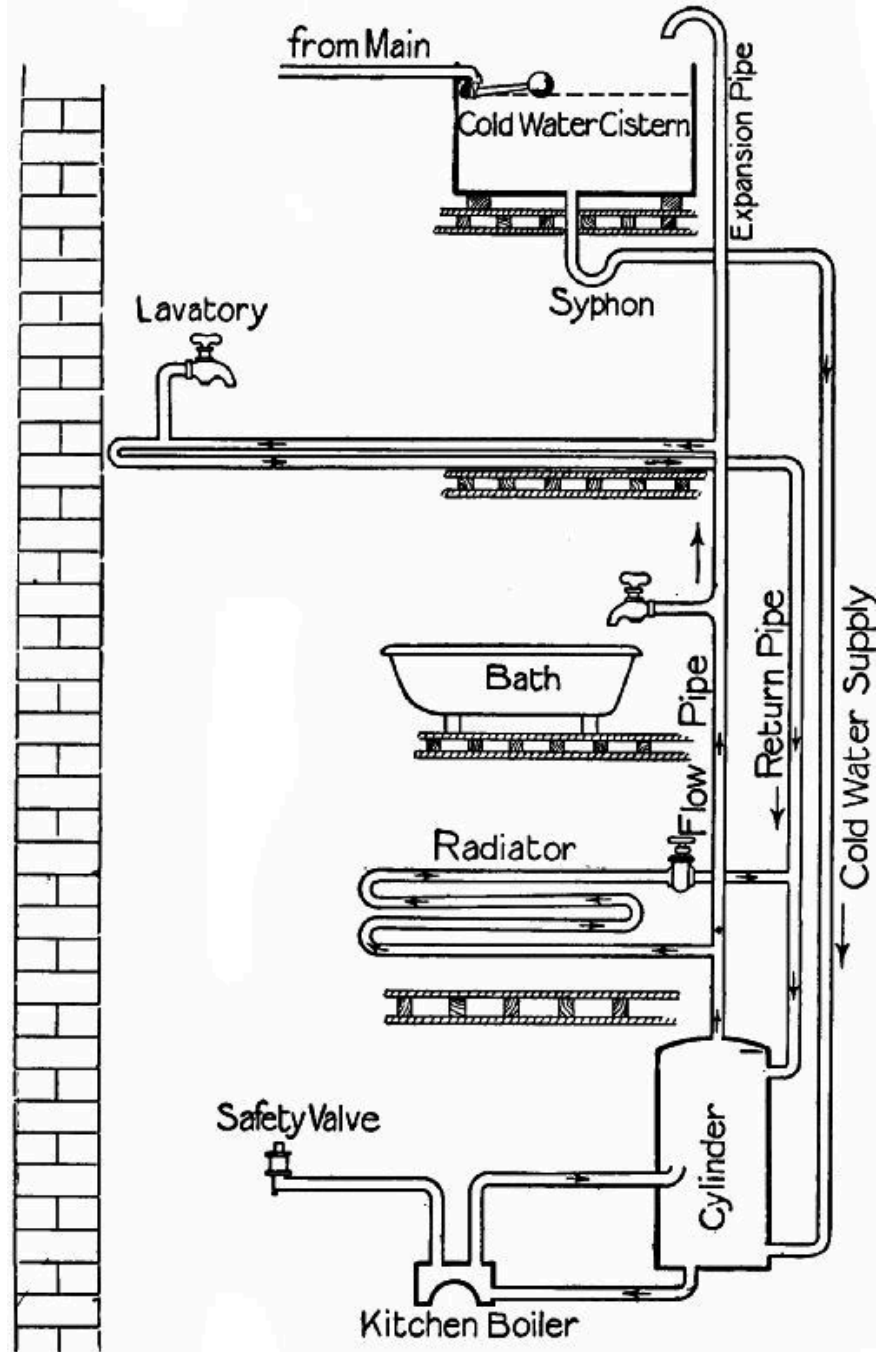
FIG. 193.—The "cylinder" system of hot-water supply.
