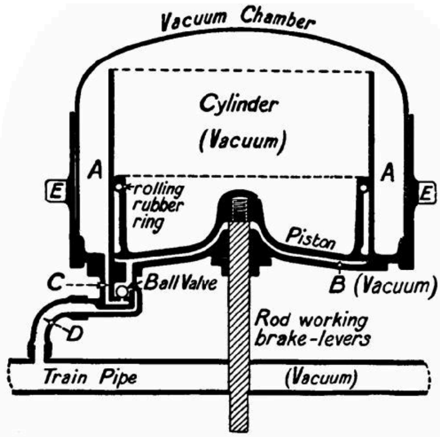
FIG. 85.—Vacuum brake "off."
