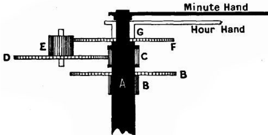
FIG. 211.—The hour-hand train of a clock.
