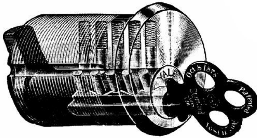
FIG. 220.—Yale key turning.
