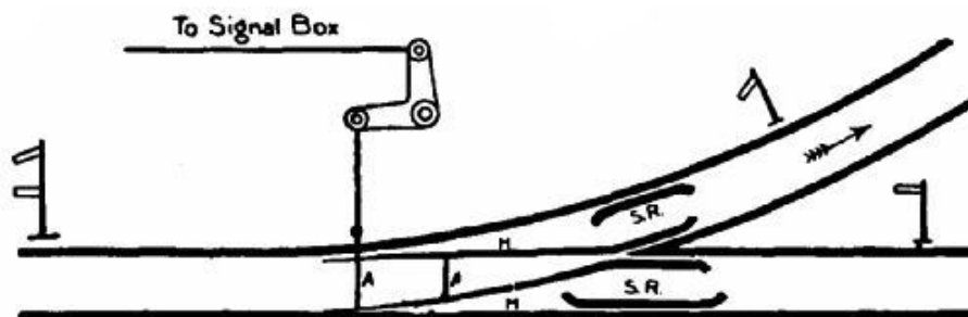
FIG. 99.—Points open to branch line.
