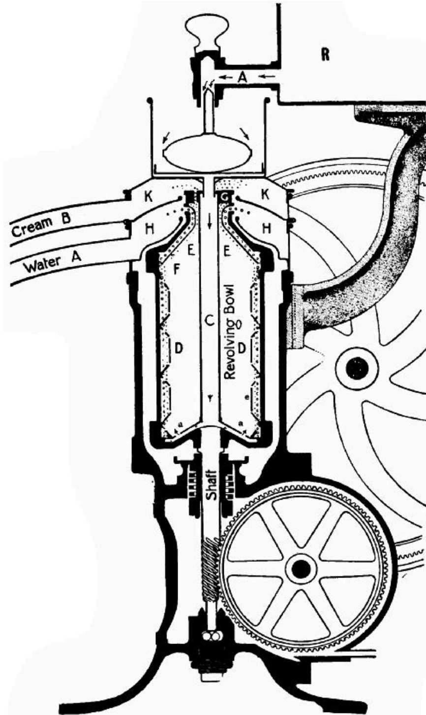
FIG. 191.—Section of a Cream Separator.
