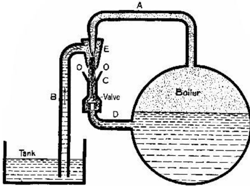
FIG. 15.—Diagram illustrating the principle of a steam-injector.
