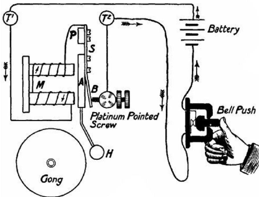
FIG. 52.—Sketch of an electric-bell circuit.
