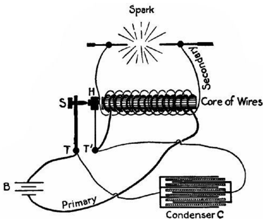
FIG. 53.—Sketch of an induction coil.
