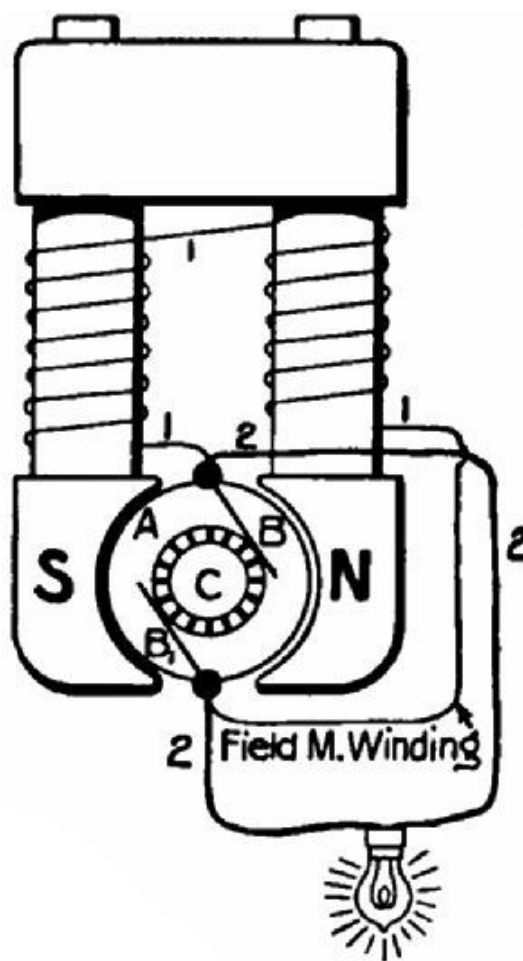
FIG. 78.—"Shunt" winding.
