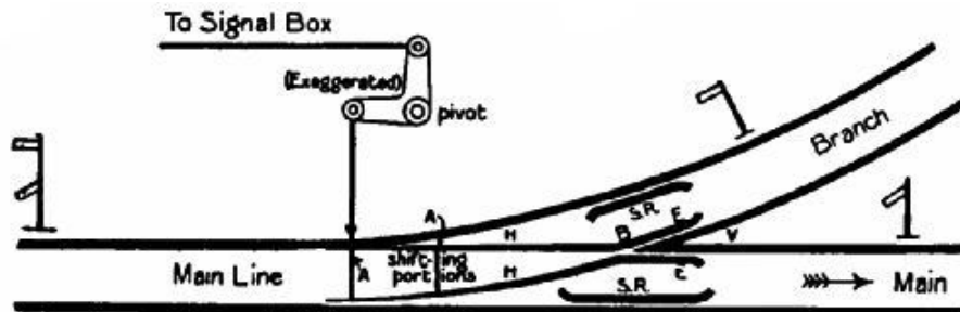
FIG. 98.—Points open to main line.
