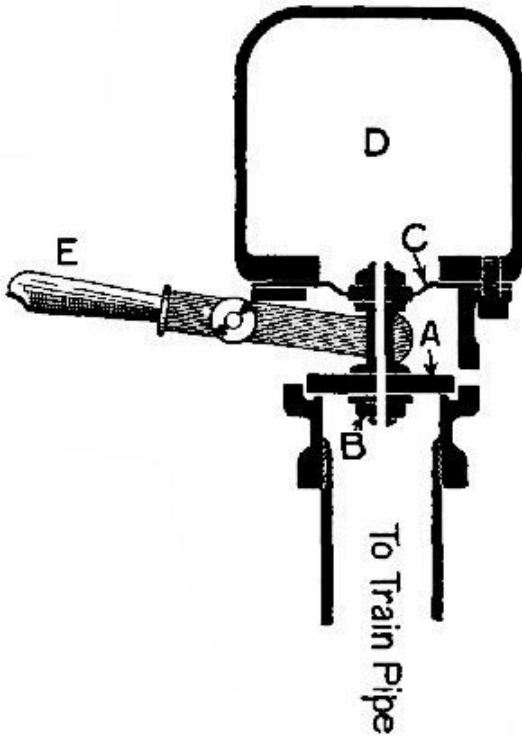
FIG. 87.—Guard's valve for applying the Vacuum brake.
