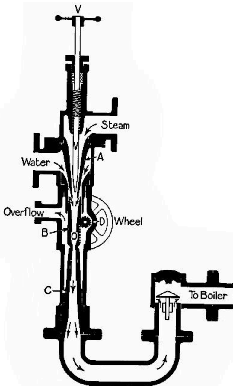
FIG. 16.—The Giffard injector.
