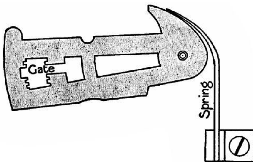
FIG. 216.—Tumbler of Chubb lock.
