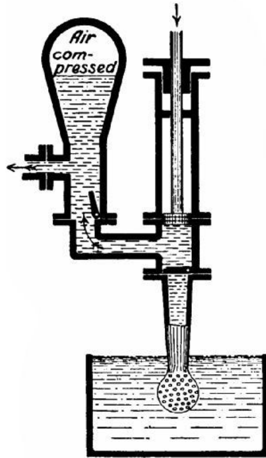
FIG. 176. Force-pump; delivery stroke.
