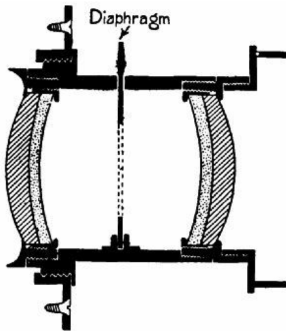
FIG. 115.—Section of a rectilinear lens.
