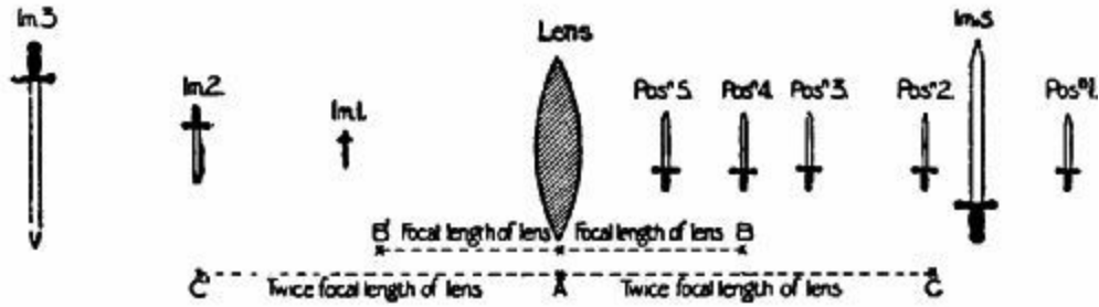
FIG. 110.—Showing how the position of the image alters relatively to the position of the object.
