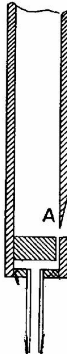
FIG. 138.—Section of an ordinary wooden "flue" pipe.
