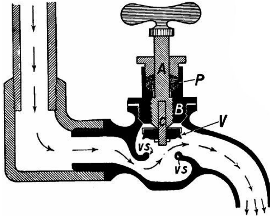
FIG. 181.—A screw-down water cock.
