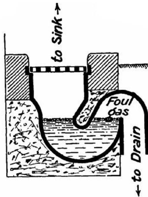
FIG. 186.—A trap for foul air.
