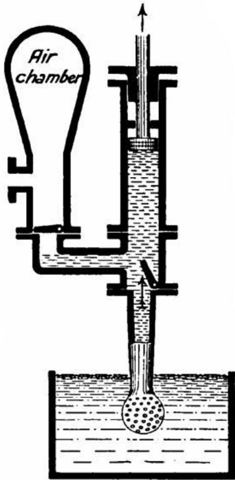
FIG. 175. Force-pump; suction stroke.
