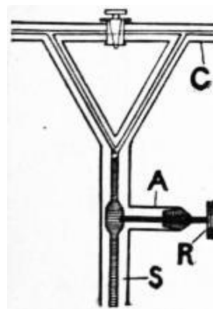
FIG. 17.—Cuccatti's Thermo-Regulator.
