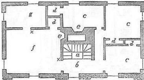
Fig. 24. Second Story.
