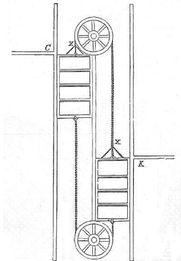
C, Parlor ceiling. K, Kitchen ceiling.
