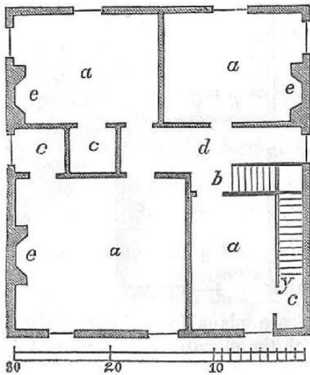
Fig. 28. Second Story.
