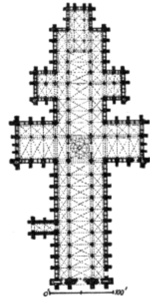
FIG. 128.—PLAN OF SALISBURY CATHEDRAL.
