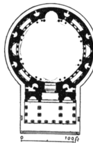
FIG. 54.—PLAN OF THE PANTHEON.
