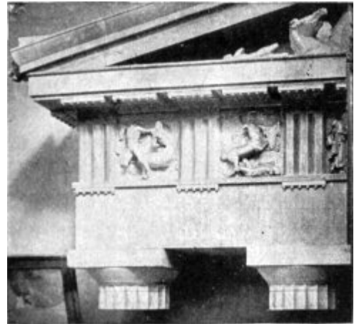
FIG. 27.—DORIC ORDER OF THE PARTHENON.
