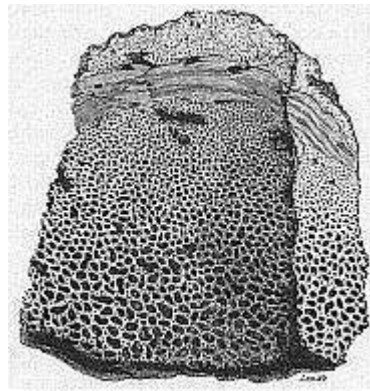
Cellular formation of volcanic bomb
