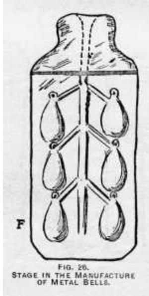
FIG. 26. STAGES IN THE MANUFACTURE OF METAL BELLS.
