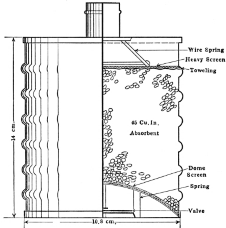
FIG. 65.—Ammonia Canister—"Kupramite."
