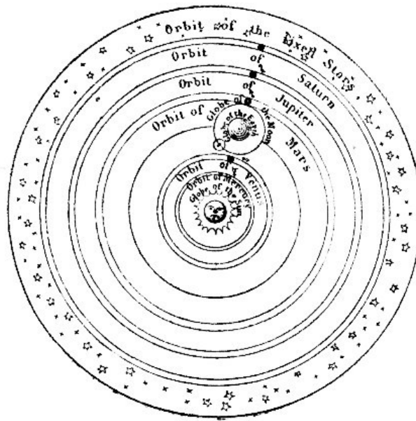
FIG. 20.—THE COPERNICAN SYSTEM.
