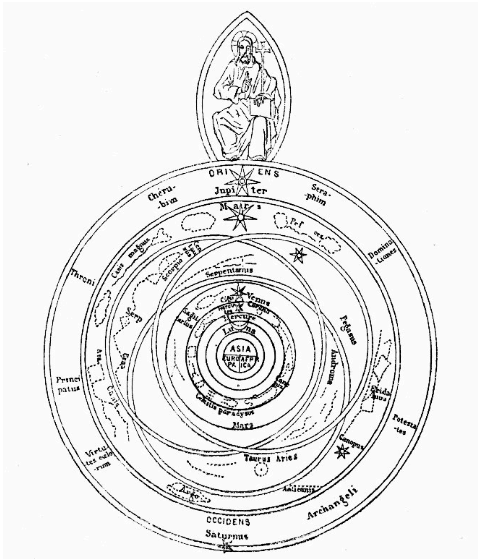
FIG. 16.—HEAVENS OF THE MIDDLE AGES.
