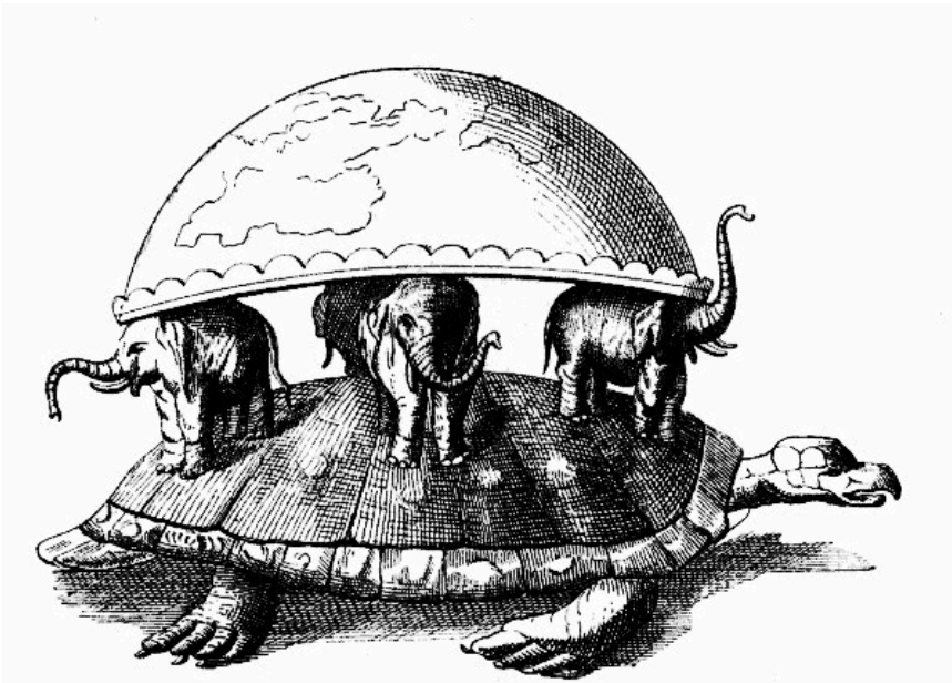
FIG. 28.—HINDOO EARTH.
