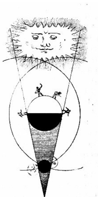
FIG. 35.—THE EARTH'S SHADOW.
