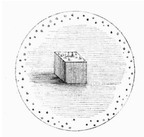
FIG. 30.—PLATO'S CUBICAL EARTH.
