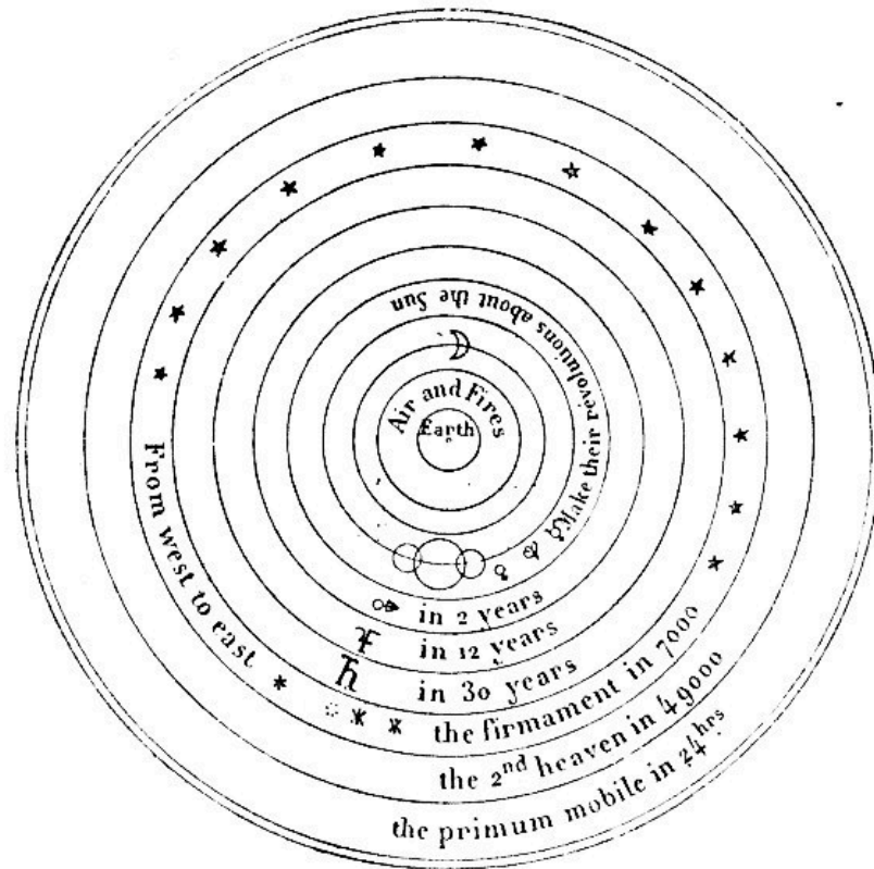
FIG. 19.—CAPELLA'S SYSTEM.
