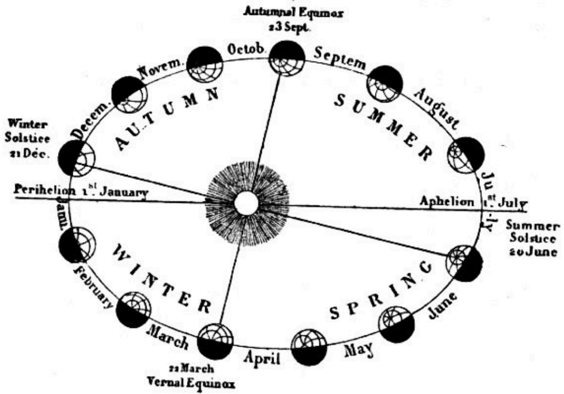
THE EARTH'S YEAR, AND THE MONTHS.
