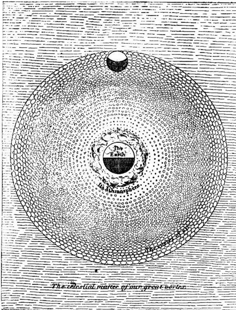
FIG. 22.—DESCARTES' THEORY OF VORTICES.
