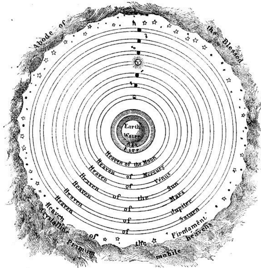
FIG. 14.—PTOLEMY'S ASTRONOMICAL SYSTEM.
