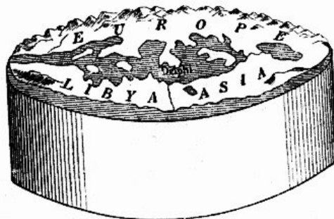
FIG. 29.—THE EARTH OF ANAXIMANDER.
