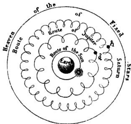
FIG. 15.—THE EPICYCLES OF PTOLEMY.
