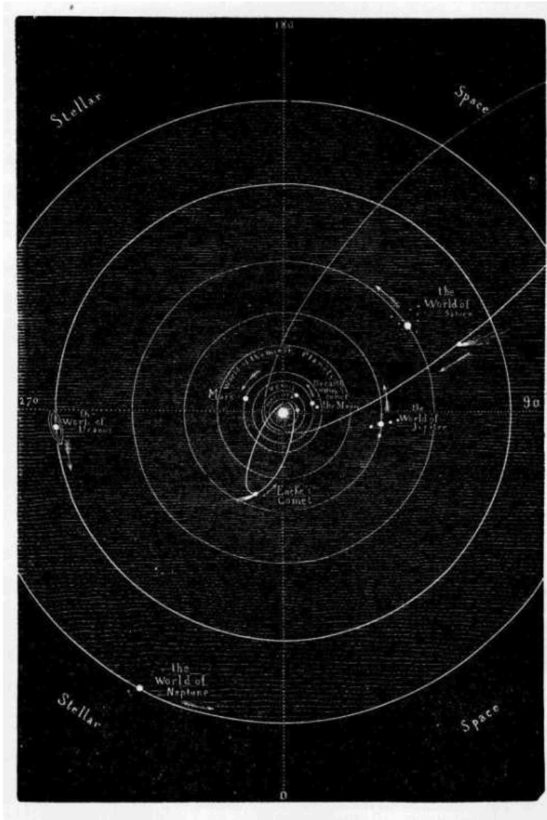
PLATE IX.—THE SOLAR SYSTEM.
