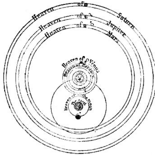
FIG. 21.—TYCHO BRAHE'S SYSTEM.
