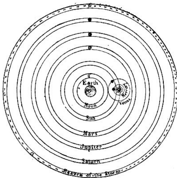
FIG. 18.—EGYPTIAN SYSTEM.
