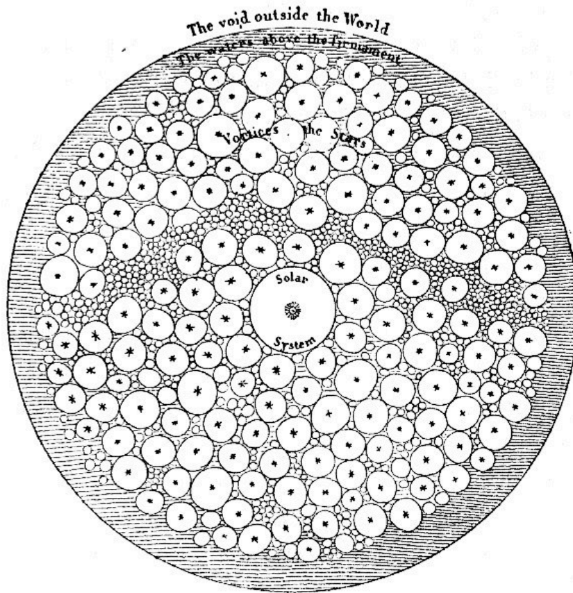
FIG. 23.—VORTICES OF THE STARS.
