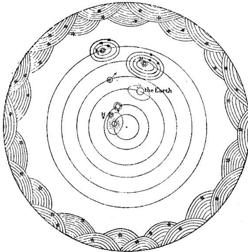
FIG. 24.—VARIATION OF DESCARTES' THEORY.
