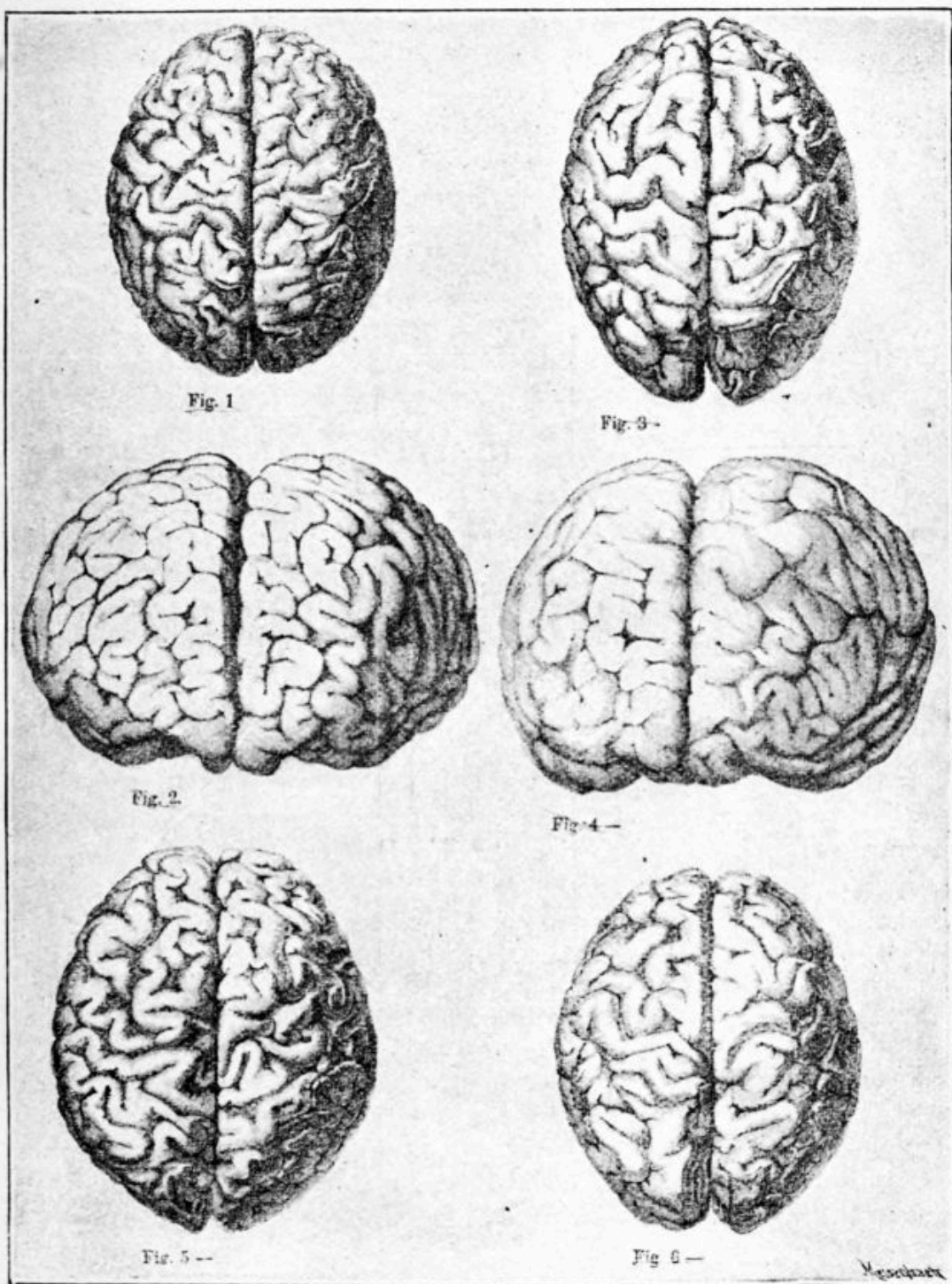
Fig. 1. Gauss's Brain.
