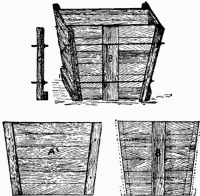
138. Box for transporting large transplanted stock.
