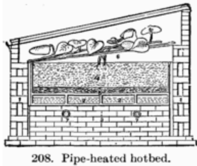
208. Pipe-heated hotbed.
