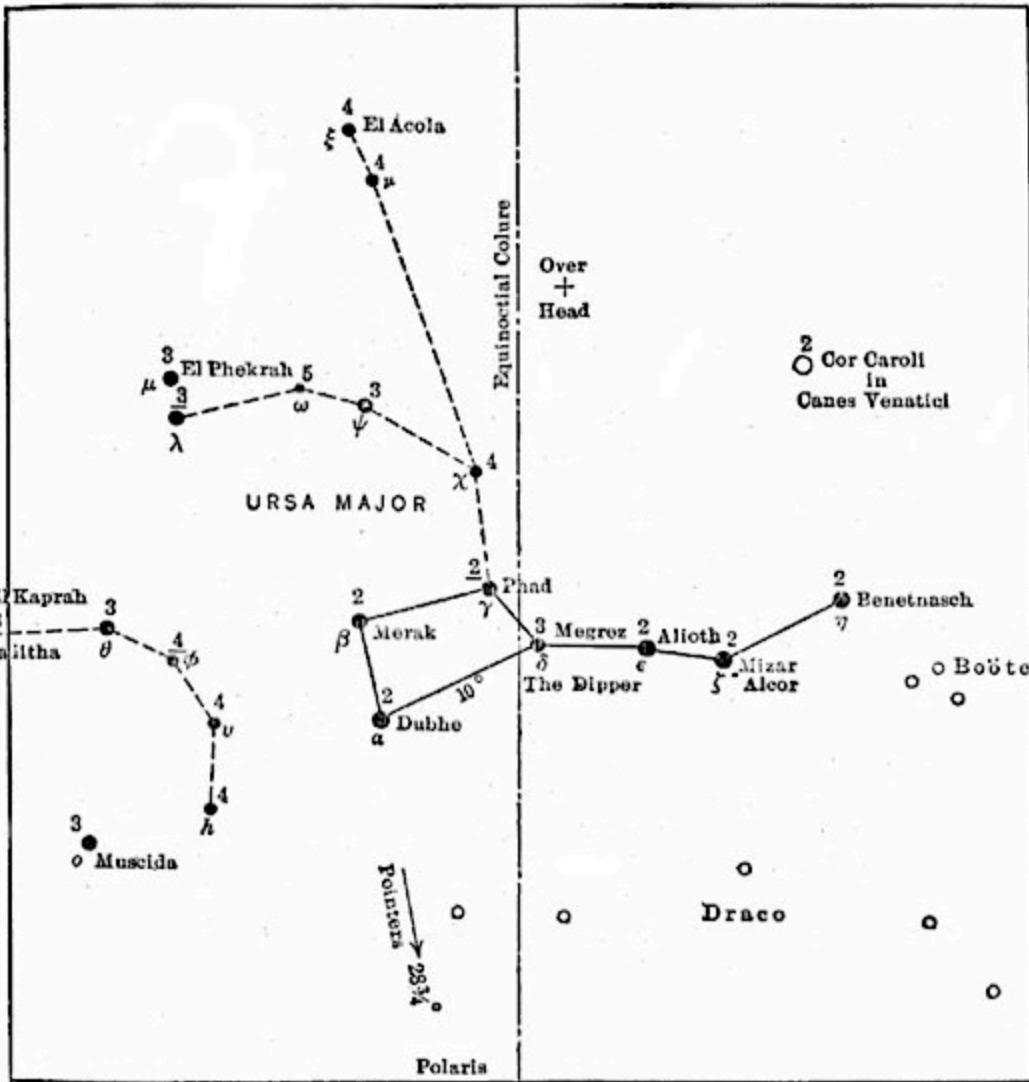
URSA MAJOR
