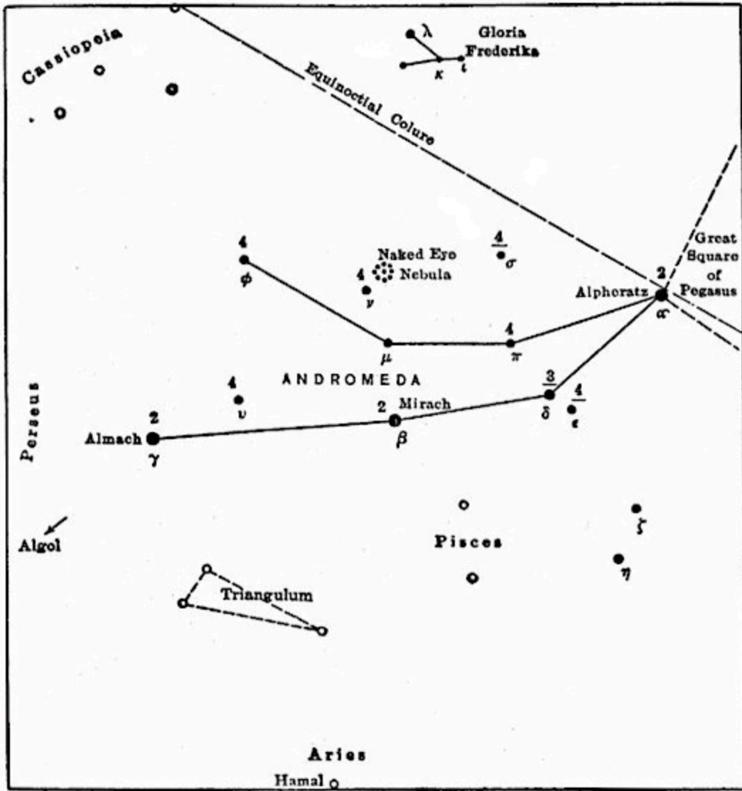
ANDROMEDA
