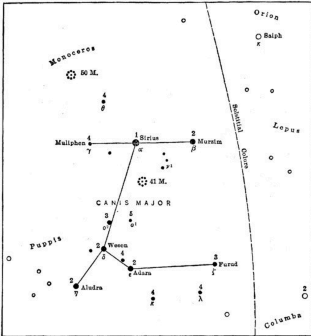
CANIS MAJOR
