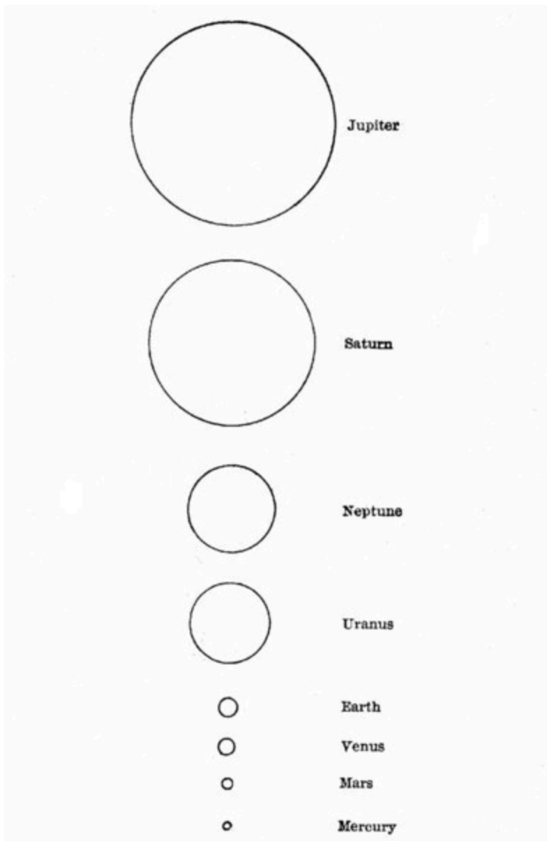
COMPARATIVE SIZE OF THE PLANETS.
