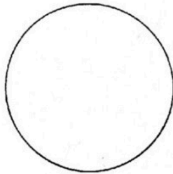
Saturn
