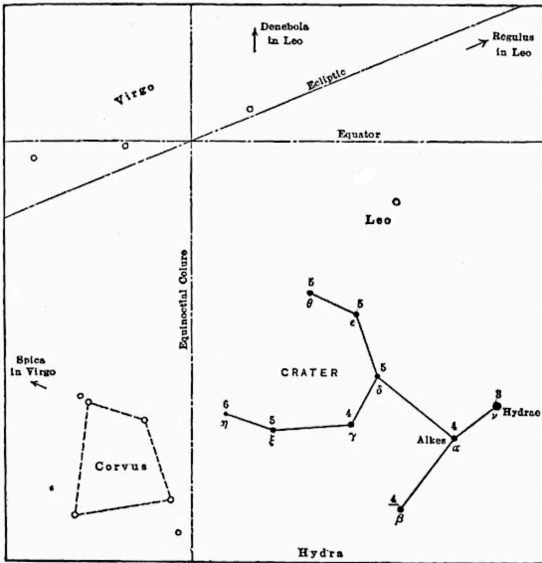
CRATER
