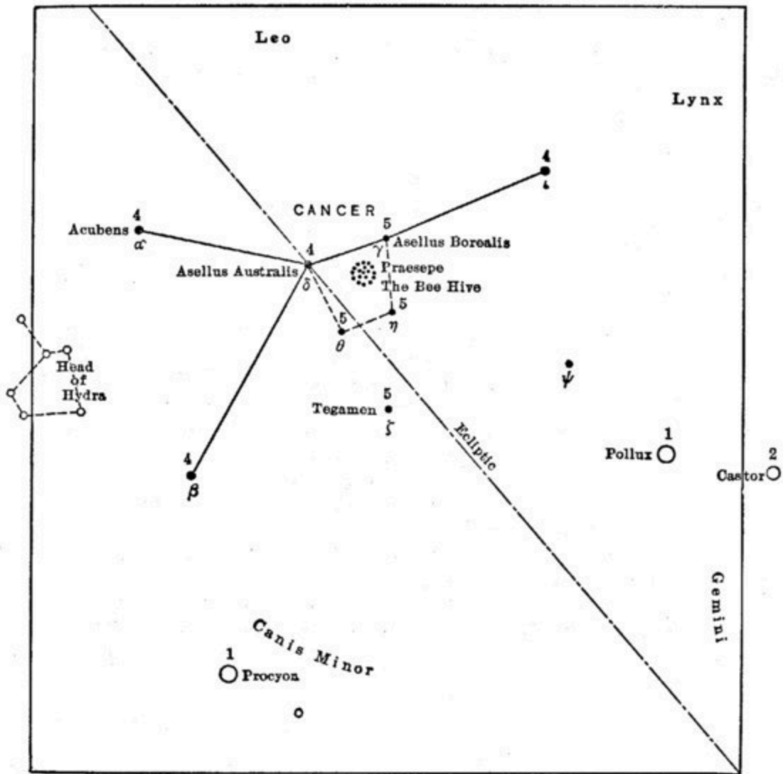
CANCER
