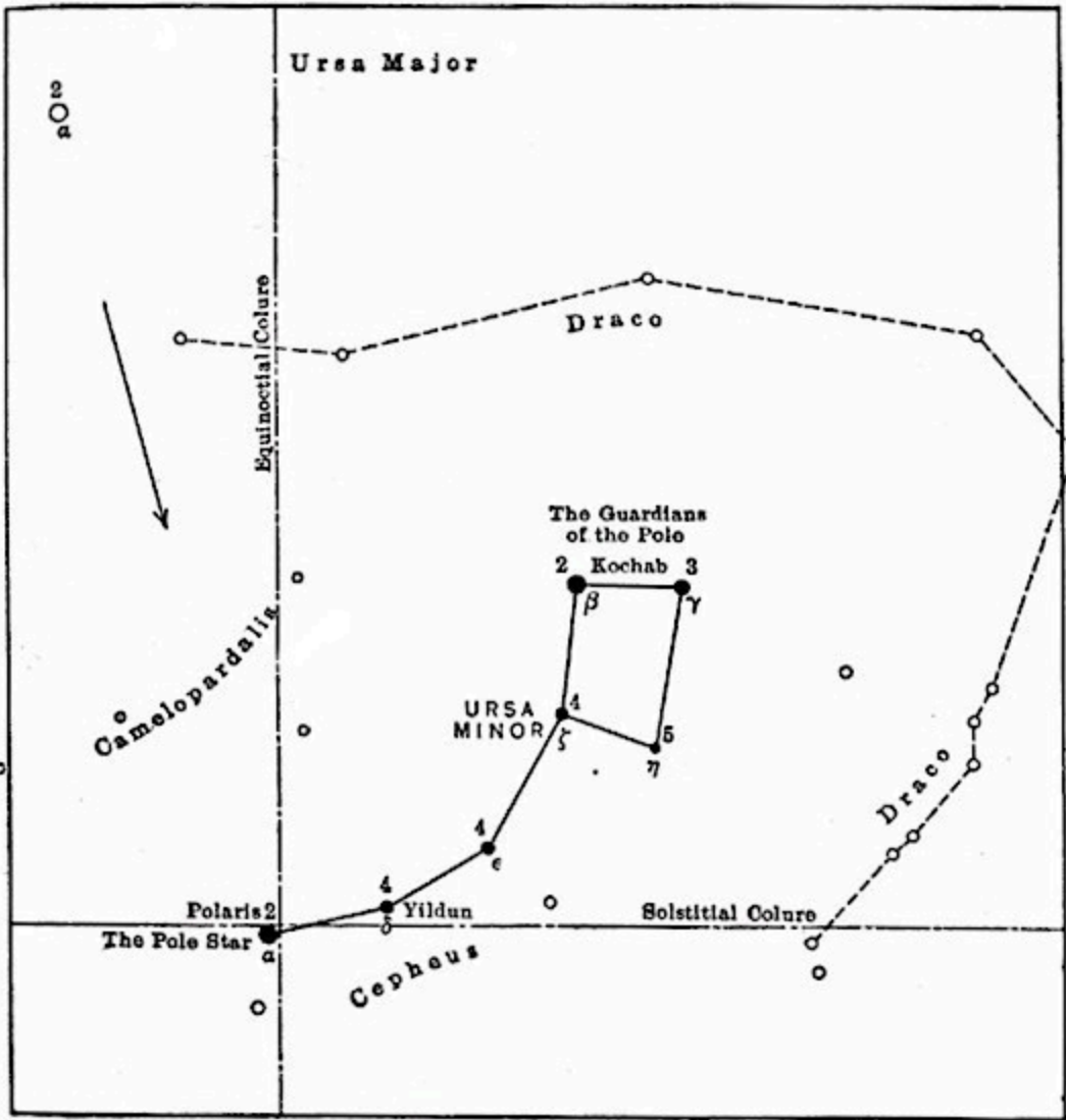
URSA MINOR
