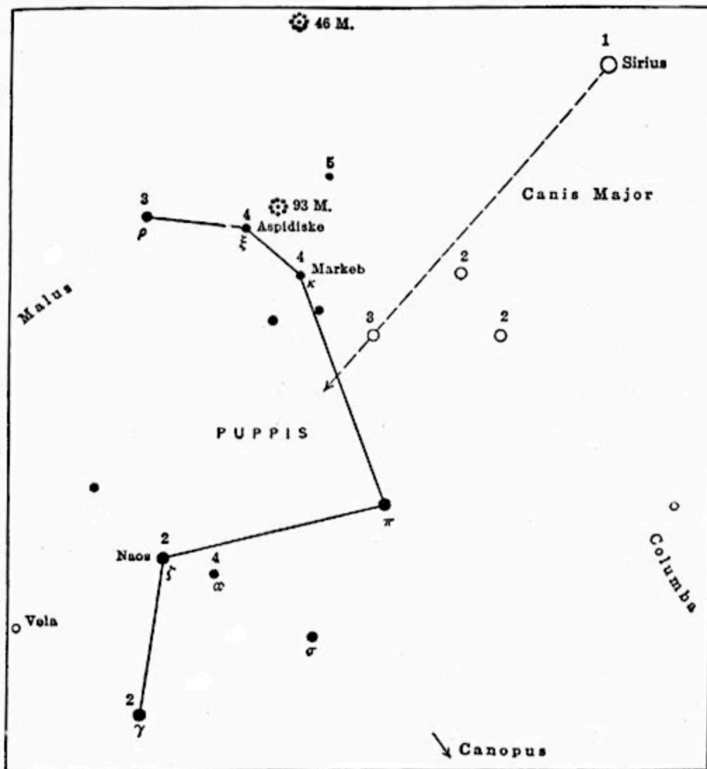
PUPPIS
