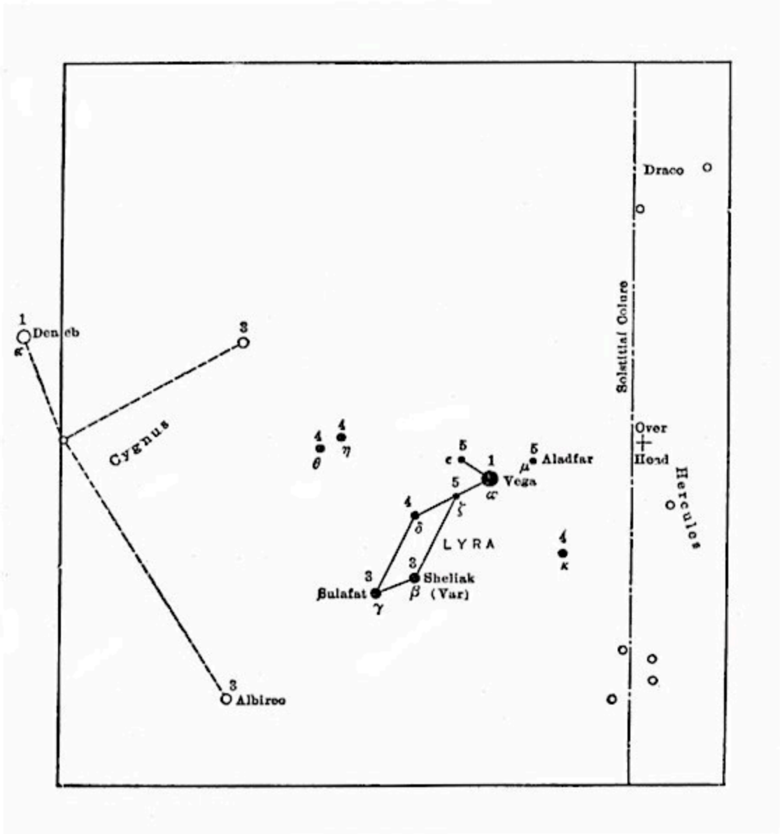
LYRA
