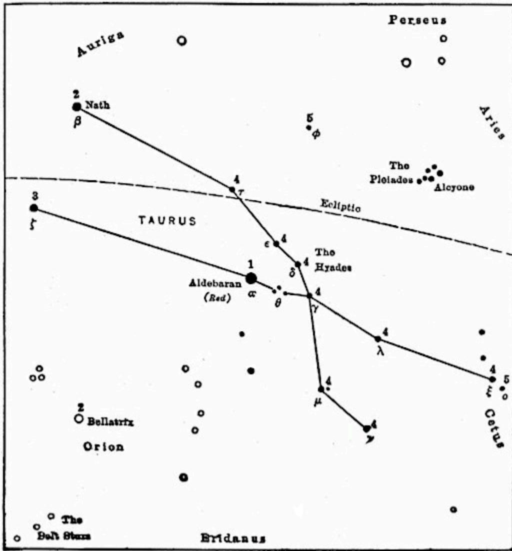
TAURUS
