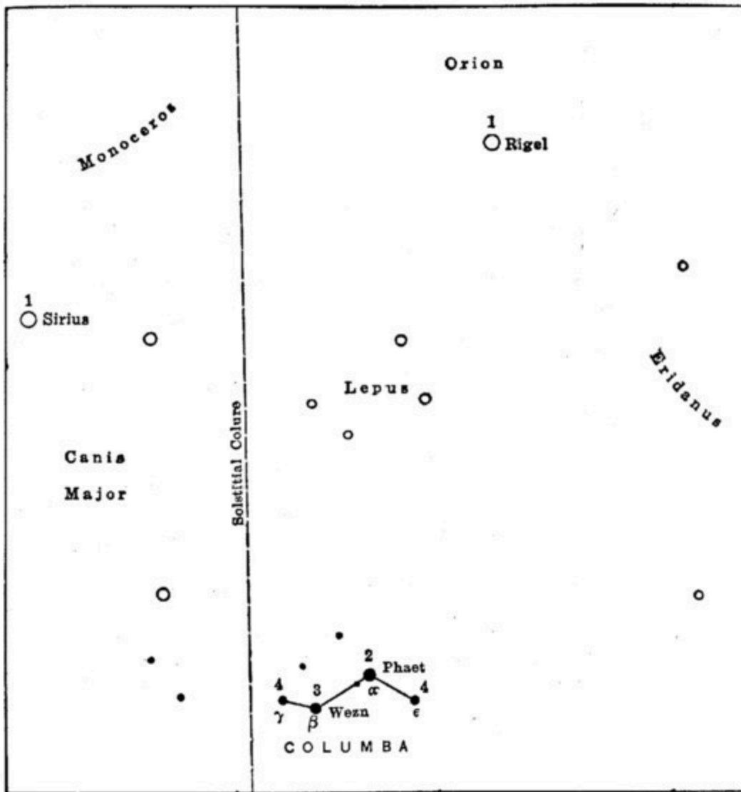
COLUMBA
