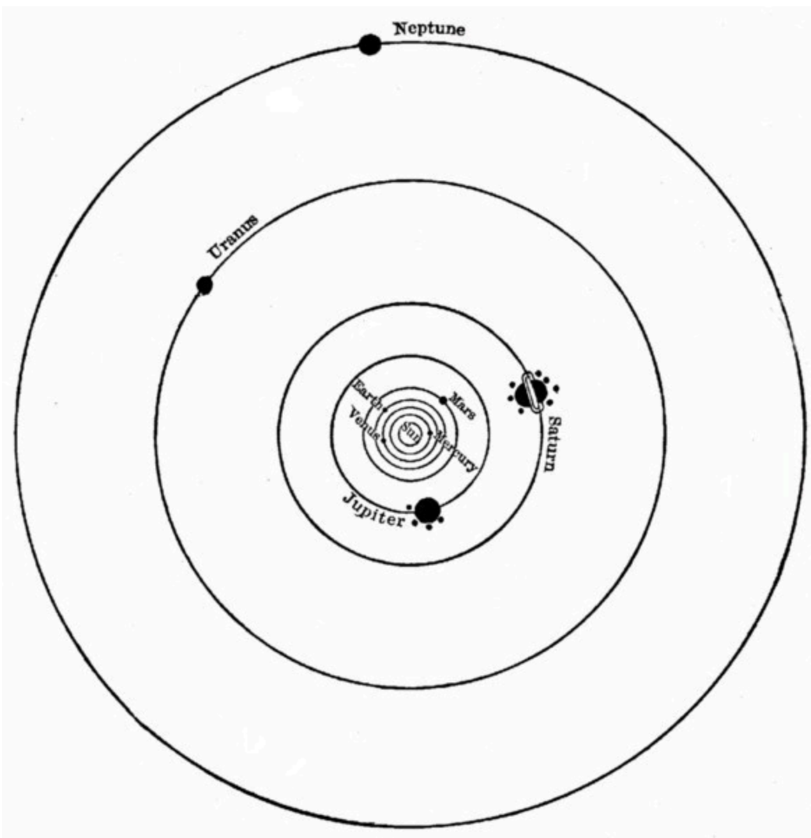
THE PLANETARY ORBITS
