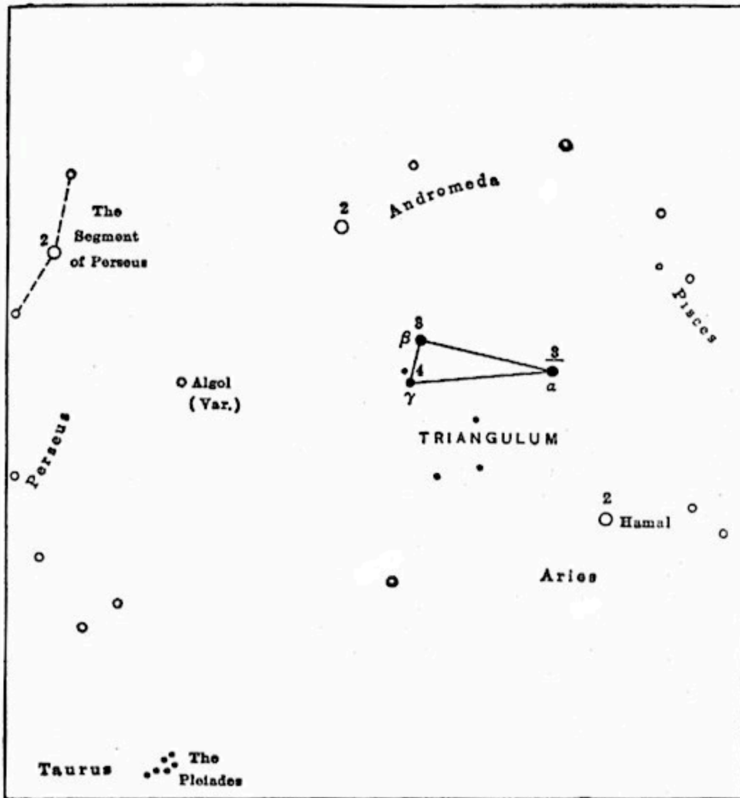
TRIANGULUM
