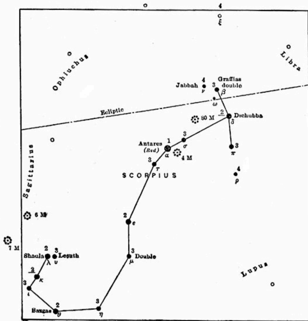
SCORPIUS
