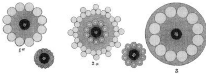
SECTIONS OF CABLES (REDUCED). 1. Main cable of 1858. 1a. Shore end, abandoned cable of 1858. 2. Main cable of 1866. 2a. Shore-end, recovered cable of 1865. 3. Shore end of cable of 1866.
